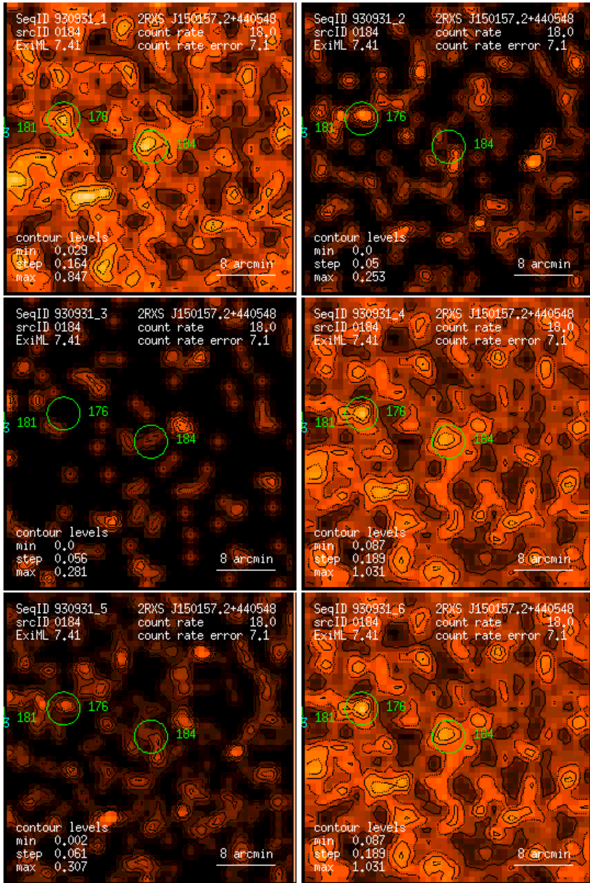
Figure 184: RASS 930931: detection 0184: band rate images, Gaussian filter: (1) PSPC channels 11 – 41, (2) 52 – 90, (3) 91 – 201, (4) 11 – 235, (5) 52 – 201, (6) 11 – 201. Broad band rates in counts/ks. Band rate contour levels in counts/ks/arcmin 2 .
