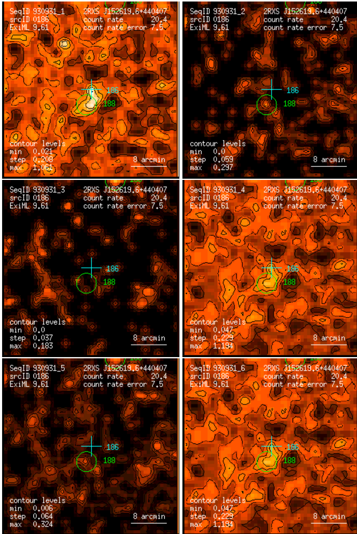
Figure 186: RASS 930931: detection 0186: band rate images, Gaussian filter: (1) PSPC channels 11 – 41, (2) 52 – 90, (3) 91 – 201, (4) 11 – 235, (5) 52 – 201, (6) 11 – 201. Broad band rates in counts/ks. Band rate contour levels in counts/ks/arcmin 2 .
