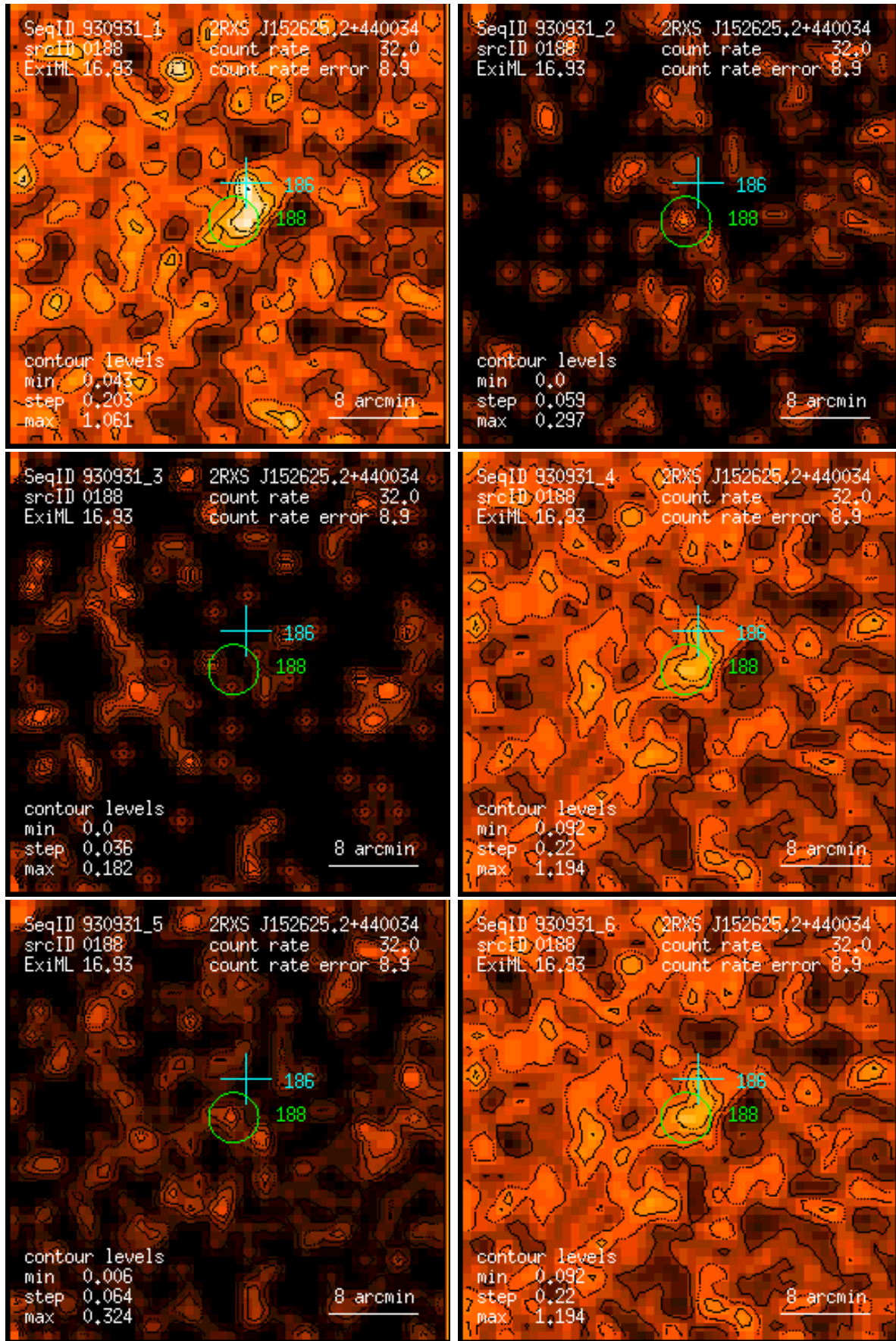
Figure 188: RASS 930931: detection 0188: band rate images, Gaussian filter: (1) PSPC channels 11 – 41, (2) 52 – 90, (3) 91 – 201, (4) 11 – 235, (5) 52 – 201, (6) 11 – 201. Broad band rates in counts/ks. Band rate contour levels in counts/ks/arcmin 2 .
