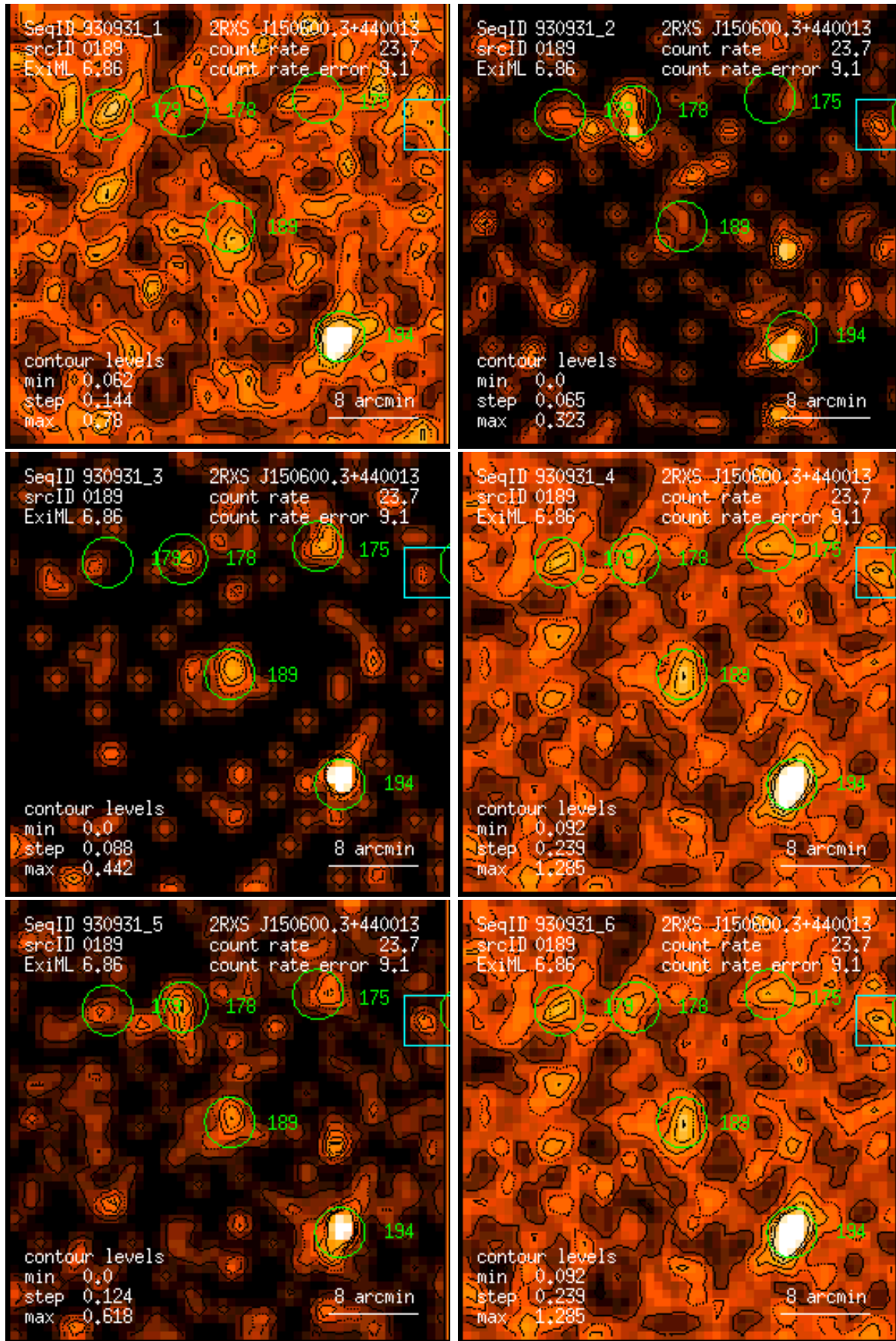
Figure 189: RASS 930931: detection 0189: band rate images, Gaussian filter: (1) PSPC channels 11 – 41, (2) 52 – 90, (3) 91 – 201, (4) 11 – 235, (5) 52 – 201, (6) 11 – 201. Broad band rates in counts/ks. Band rate contour levels in counts/ks/arcmin 2 .
