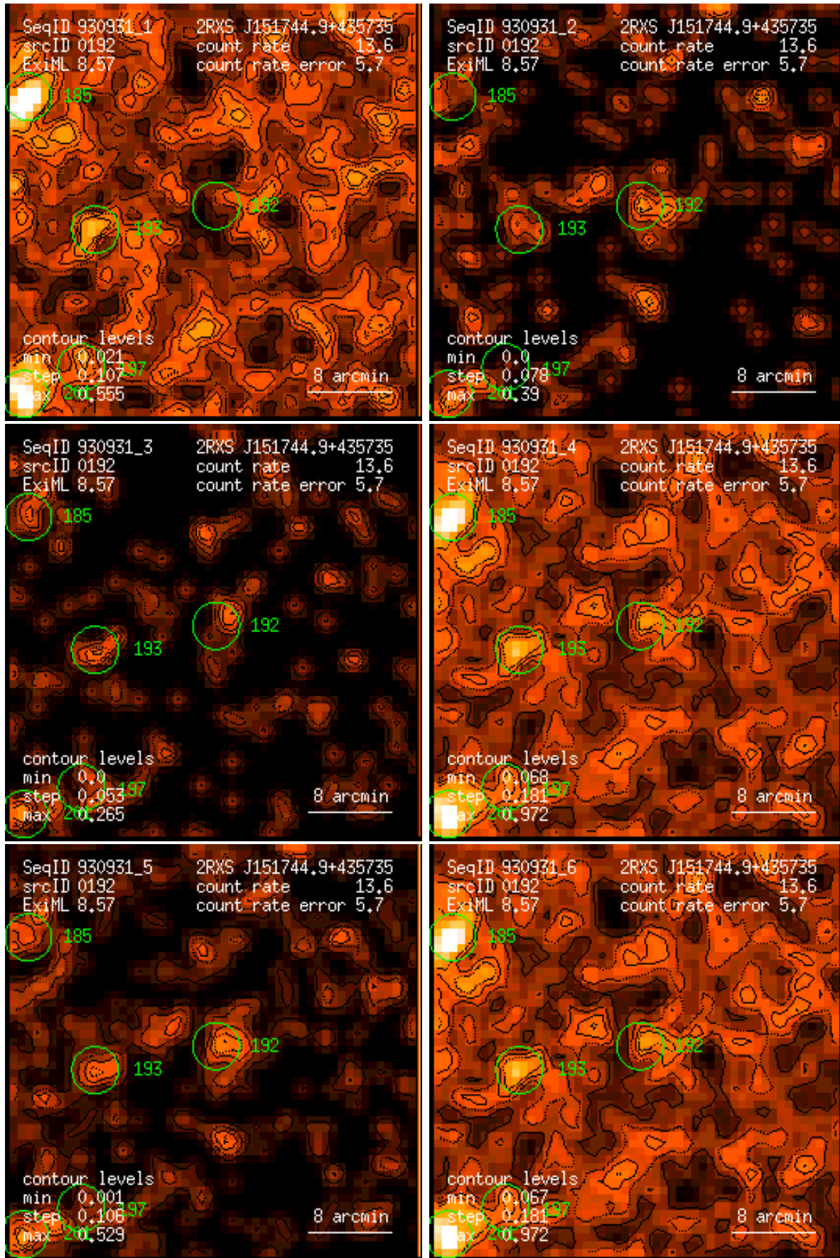
Figure 192: RASS 930931: detection 0192: band rate images, Gaussian filter: (1) PSPC channels 11 – 41, (2) 52 – 90, (3) 91 – 201, (4) 11 – 235, (5) 52 – 201, (6) 11 – 201. Broad band rates in counts/ks. Band rate contour levels in counts/ks/arcmin 2 .
