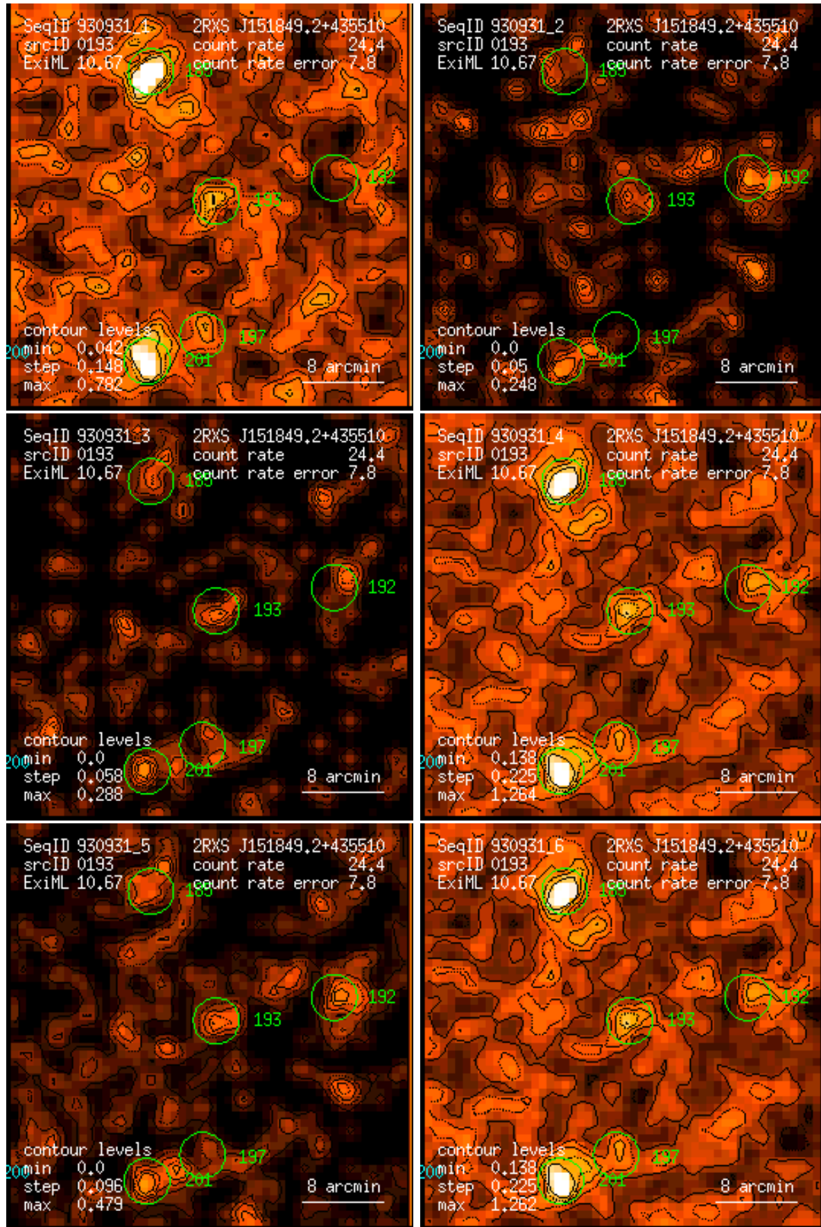
Figure 193: RASS 930931: detection 0193: band rate images, Gaussian filter: (1) PSPC channels 11 – 41, (2) 52 – 90, (3) 91 – 201, (4) 11 – 235, (5) 52 – 201, (6) 11 – 201. Broad band rates in counts/ks. Band rate contour levels in counts/ks/arcmin 2 .
