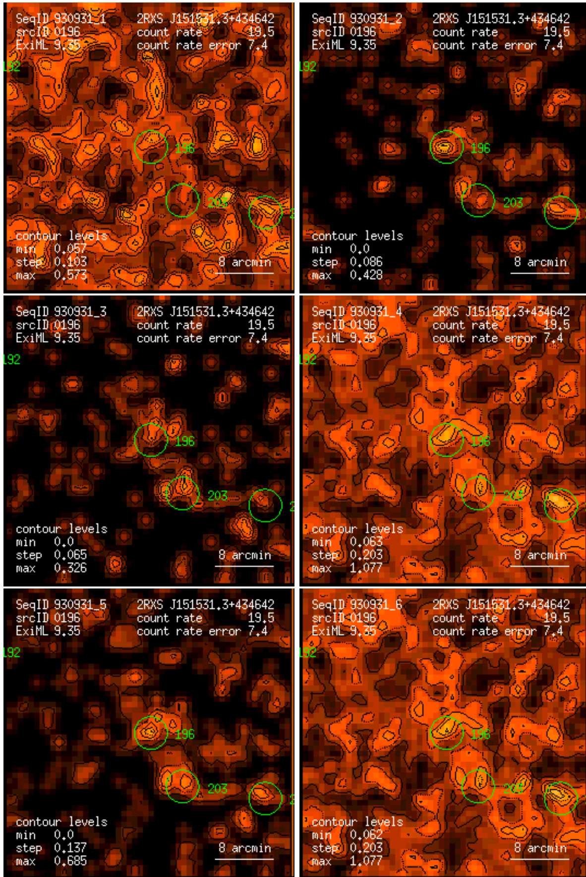
Figure 196: RASS 930931: detection 0196: band rate images, Gaussian filter: (1) PSPC channels 11 – 41, (2) 52 – 90, (3) 91 – 201, (4) 11 – 235, (5) 52 – 201, (6) 11 – 201. Broad band rates in counts/ks. Band rate contour levels in counts/ks/arcmin 2 .
