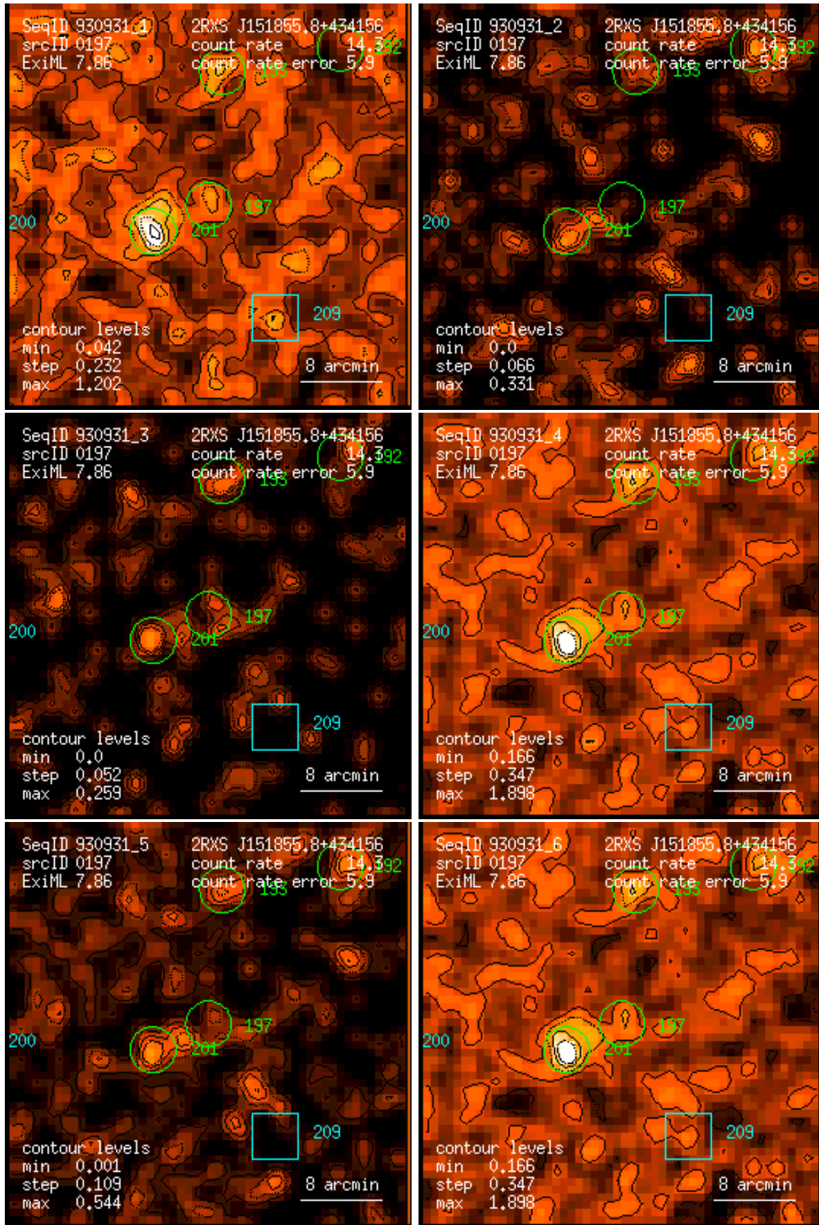
Figure 197: RASS 930931: detection 0197: band rate images, Gaussian filter: (1) PSPC channels 11 – 41, (2) 52 – 90, (3) 91 – 201, (4) 11 – 235, (5) 52 – 201, (6) 11 – 201. Broad band rates in counts/ks. Band rate contour levels in counts/ks/arcmin 2 .
