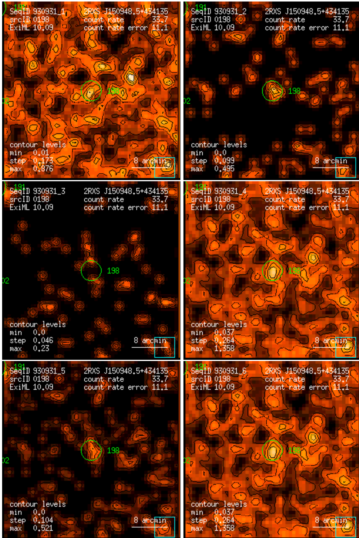
Figure 198: RASS 930931: detection 0198: band rate images, Gaussian filter: (1) PSPC channels 11 – 41, (2) 52 – 90, (3) 91 – 201, (4) 11 – 235, (5) 52 – 201, (6) 11 – 201. Broad band rates in counts/ks. Band rate contour levels in counts/ks/arcmin 2 .
