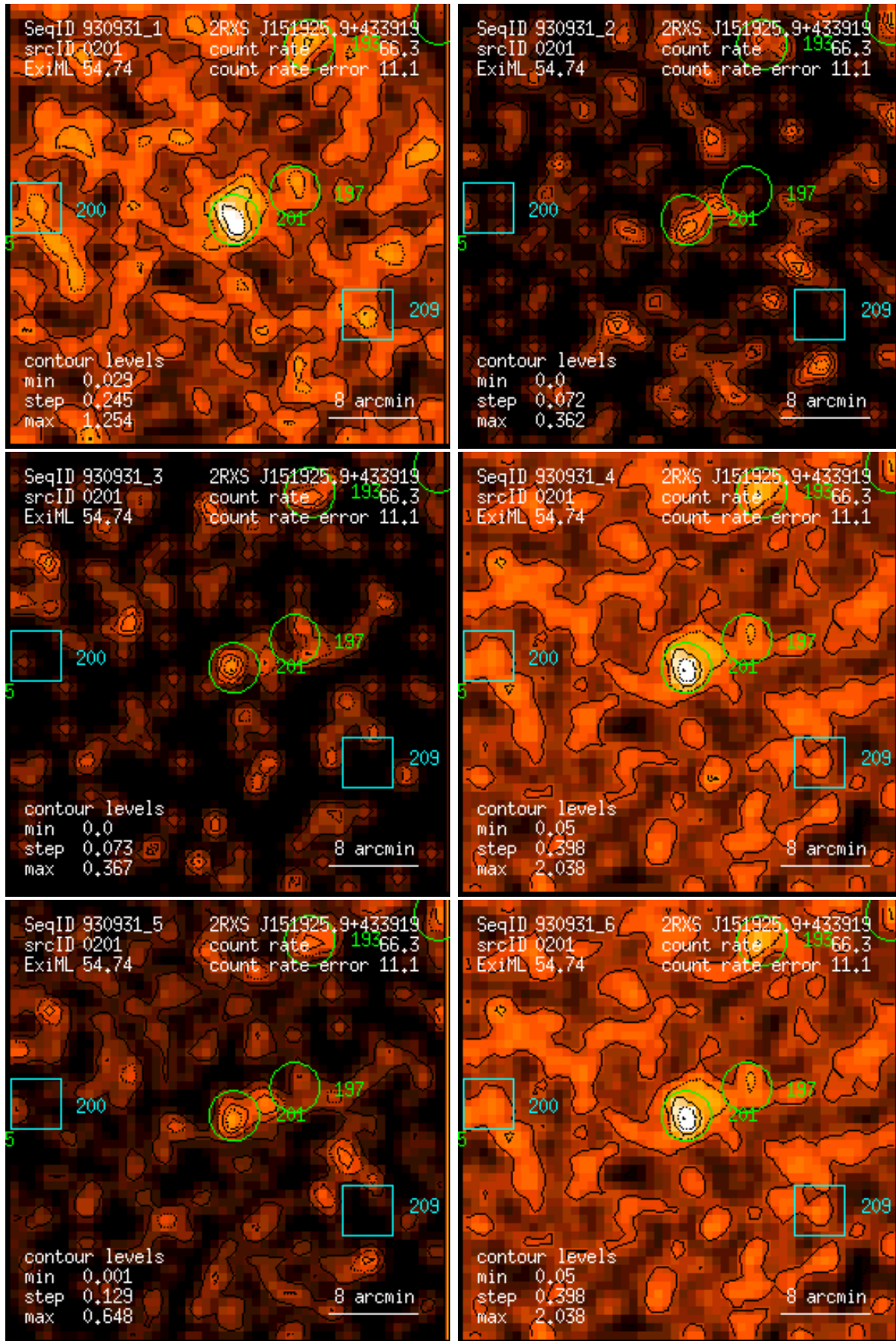
Figure 201: RASS 930931: detection 0201: band rate images, Gaussian filter: (1) PSPC channels 11 – 41, (2) 52 – 90, (3) 91 – 201, (4) 11 – 235, (5) 52 – 201, (6) 11 – 201. Broad band rates in counts/ks. Band rate contour levels in counts/ks/arcmin 2 .
