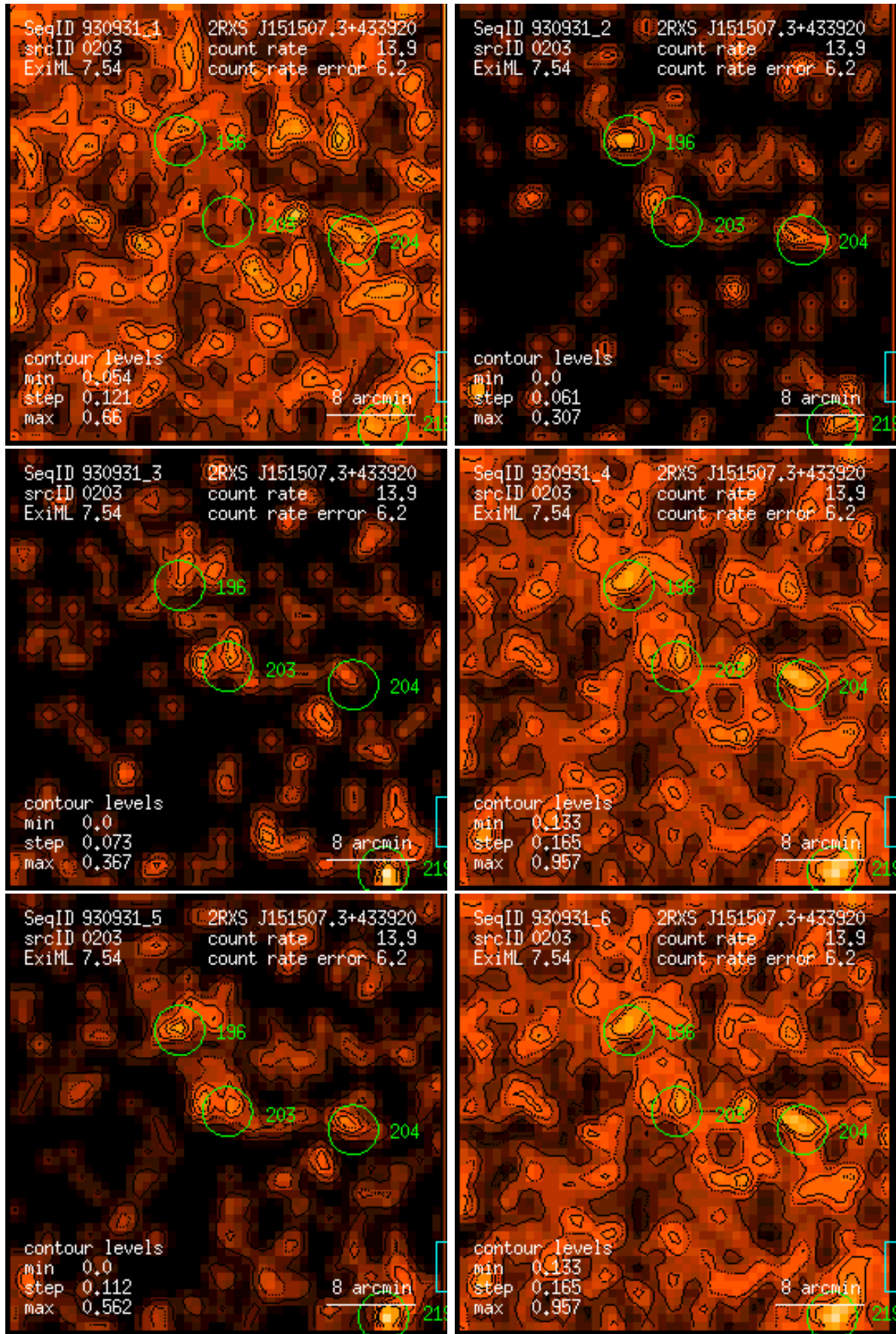
Figure 203: RASS 930931: detection 0203: band rate images, Gaussian filter: (1) PSPC channels 11 – 41, (2) 52 – 90, (3) 91 – 201, (4) 11 – 235, (5) 52 – 201, (6) 11 – 201. Broad band rates in counts/ks. Band rate contour levels in counts/ks/arcmin 2 .
