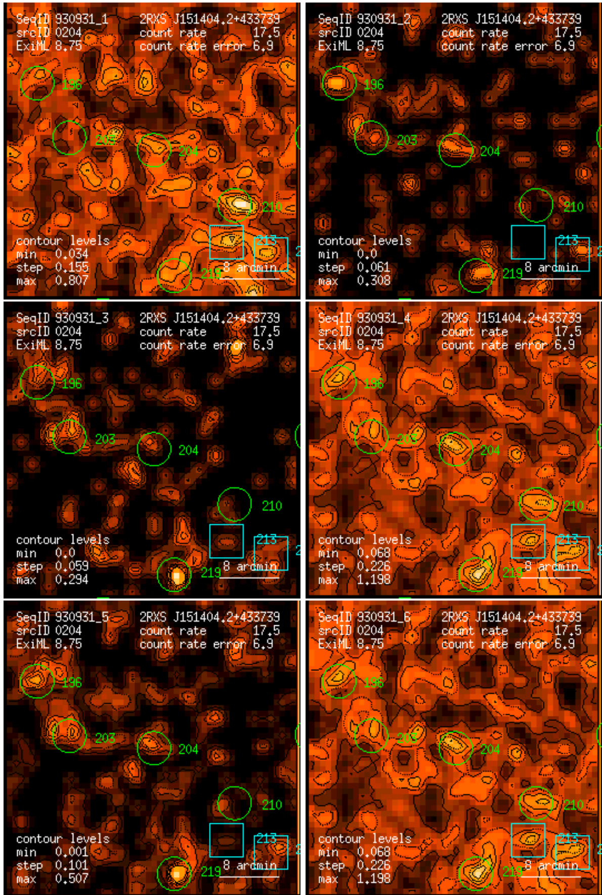
Figure 204: RASS 930931: detection 0204: band rate images, Gaussian filter: (1) PSPC channels 11 – 41, (2) 52 – 90, (3) 91 – 201, (4) 11 – 235, (5) 52 – 201, (6) 11 – 201. Broad band rates in counts/ks. Band rate contour levels in counts/ks/arcmin 2 .
