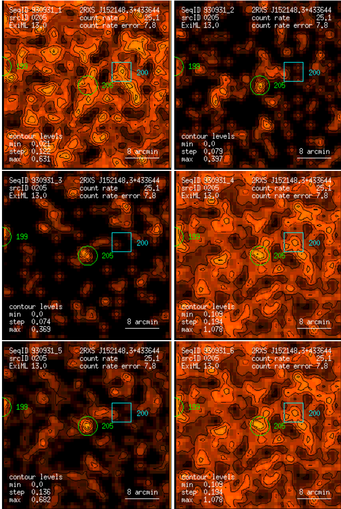
Figure 205: RASS 930931: detection 0205: band rate images, Gaussian filter: (1) PSPC channels 11 – 41, (2) 52 – 90, (3) 91 – 201, (4) 11 – 235, (5) 52 – 201, (6) 11 – 201. Broad band rates in counts/ks. Band rate contour levels in counts/ks/arcmin 2 .
