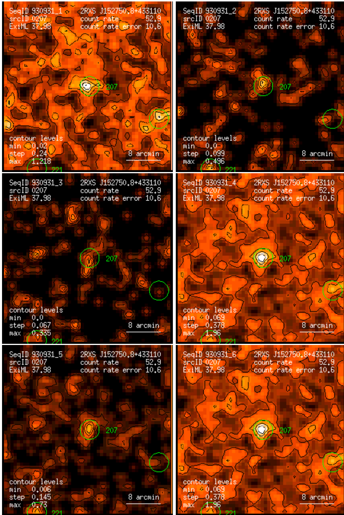
Figure 207: RASS 930931: detection 0207: band rate images, Gaussian filter: (1) PSPC channels 11 – 41, (2) 52 – 90, (3) 91 – 201, (4) 11 – 235, (5) 52 – 201, (6) 11 – 201. Broad band rates in counts/ks. Band rate contour levels in counts/ks/arcmin 2 .
