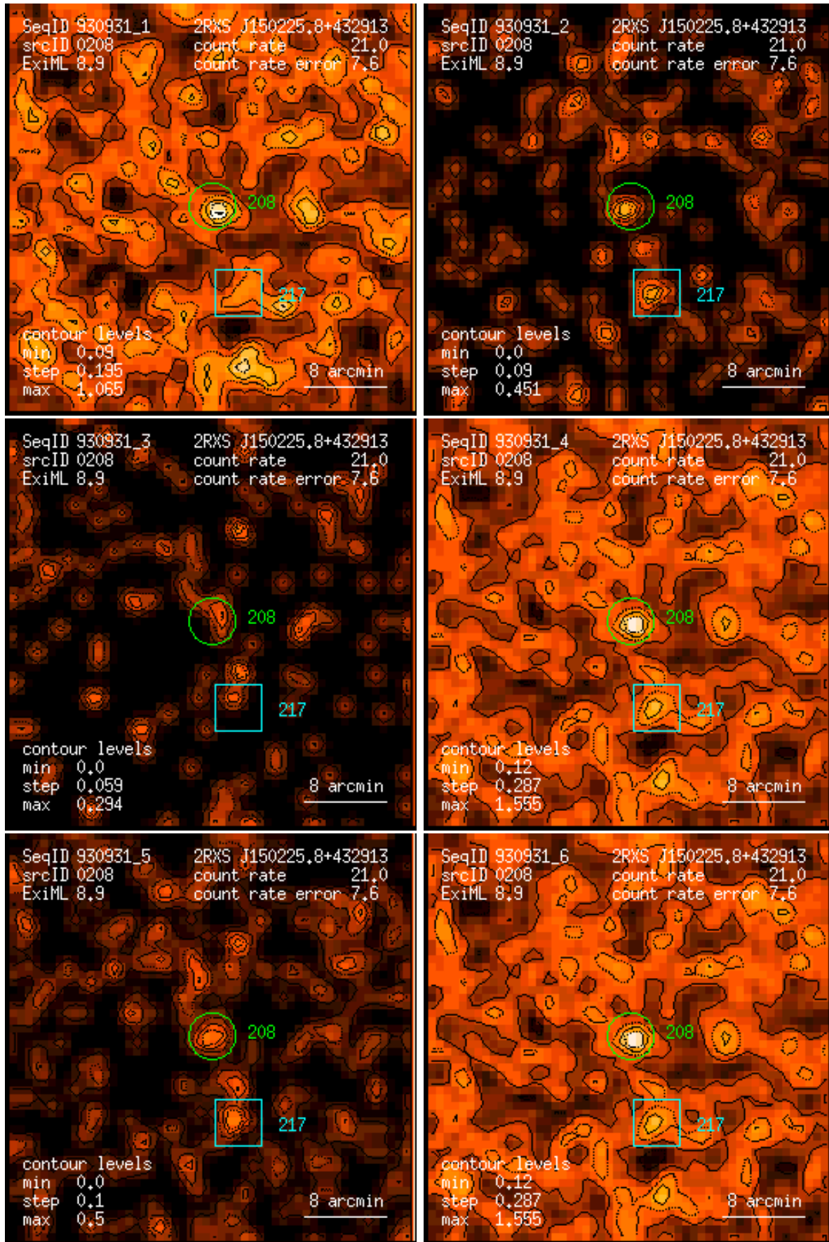
Figure 208: RASS 930931: detection 0208: band rate images, Gaussian filter: (1) PSPC channels 11 – 41, (2) 52 – 90, (3) 91 – 201, (4) 11 – 235, (5) 52 – 201, (6) 11 – 201. Broad band rates in counts/ks. Band rate contour levels in counts/ks/arcmin 2 .
