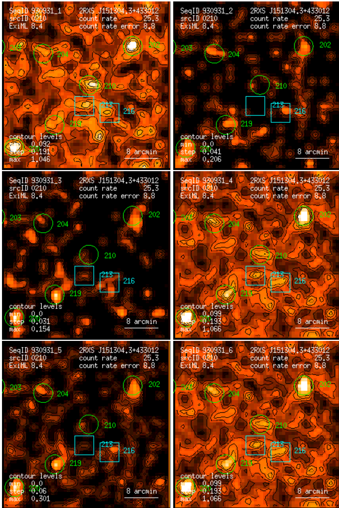
Figure 210: RASS 930931: detection 0210: band rate images, Gaussian filter: (1) PSPC channels 11 – 41, (2) 52 – 90, (3) 91 – 201, (4) 11 – 235, (5) 52 – 201, (6) 11 – 201. Broad band rates in counts/ks. Band rate contour levels in counts/ks/arcmin 2 .
