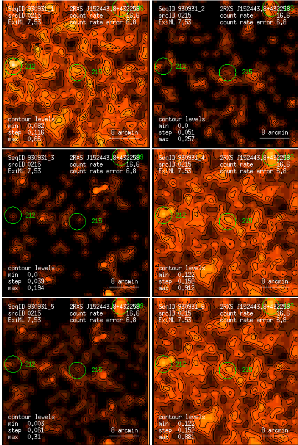
Figure 215: RASS 930931: detection 0215: band rate images, Gaussian filter: (1) PSPC channels 11 – 41, (2) 52 – 90, (3) 91 – 201, (4) 11 – 235, (5) 52 – 201, (6) 11 – 201. Broad band rates in counts/ks. Band rate contour levels in counts/ks/arcmin 2 .
