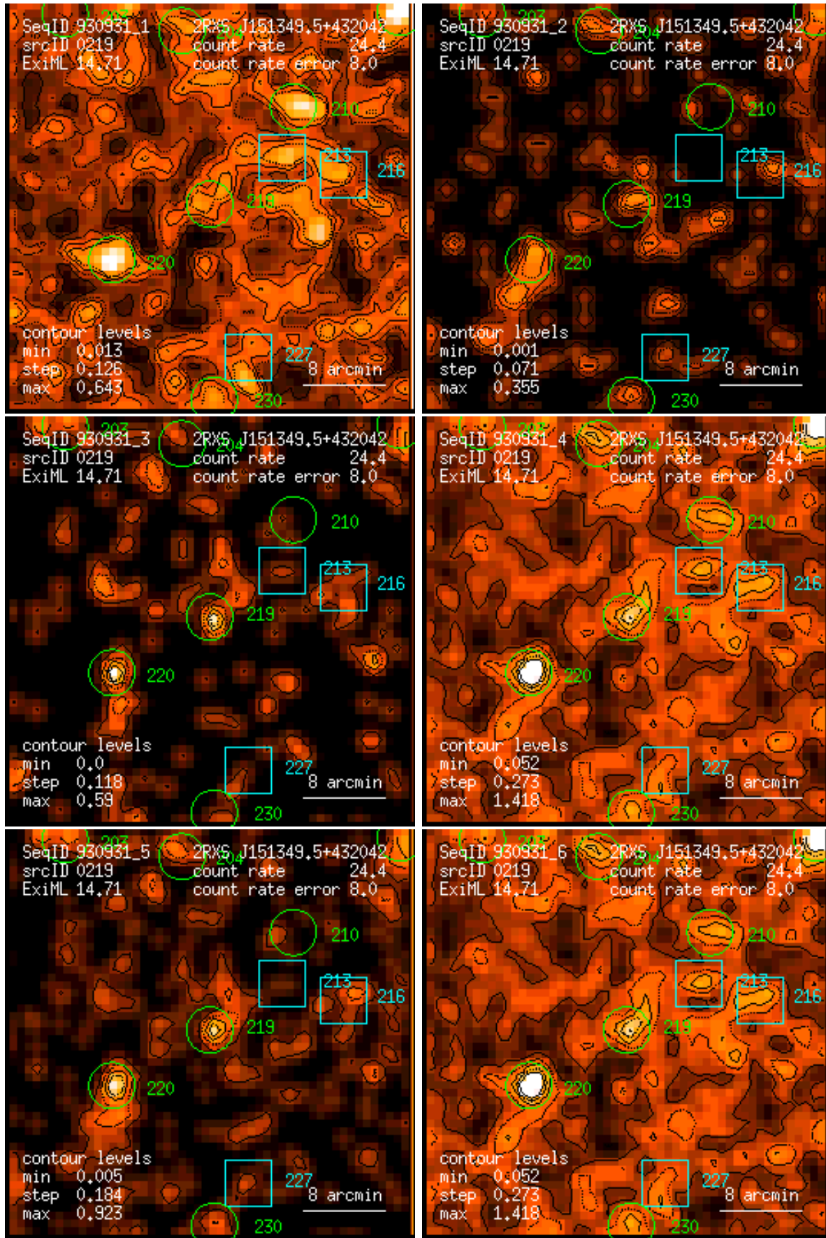
Figure 219: RASS 930931: detection 0219: band rate images, Gaussian filter: (1) PSPC channels 11 – 41, (2) 52 – 90, (3) 91 – 201, (4) 11 – 235, (5) 52 – 201, (6) 11 – 201. Broad band rates in counts/ks. Band rate contour levels in counts/ks/arcmin 2 .
