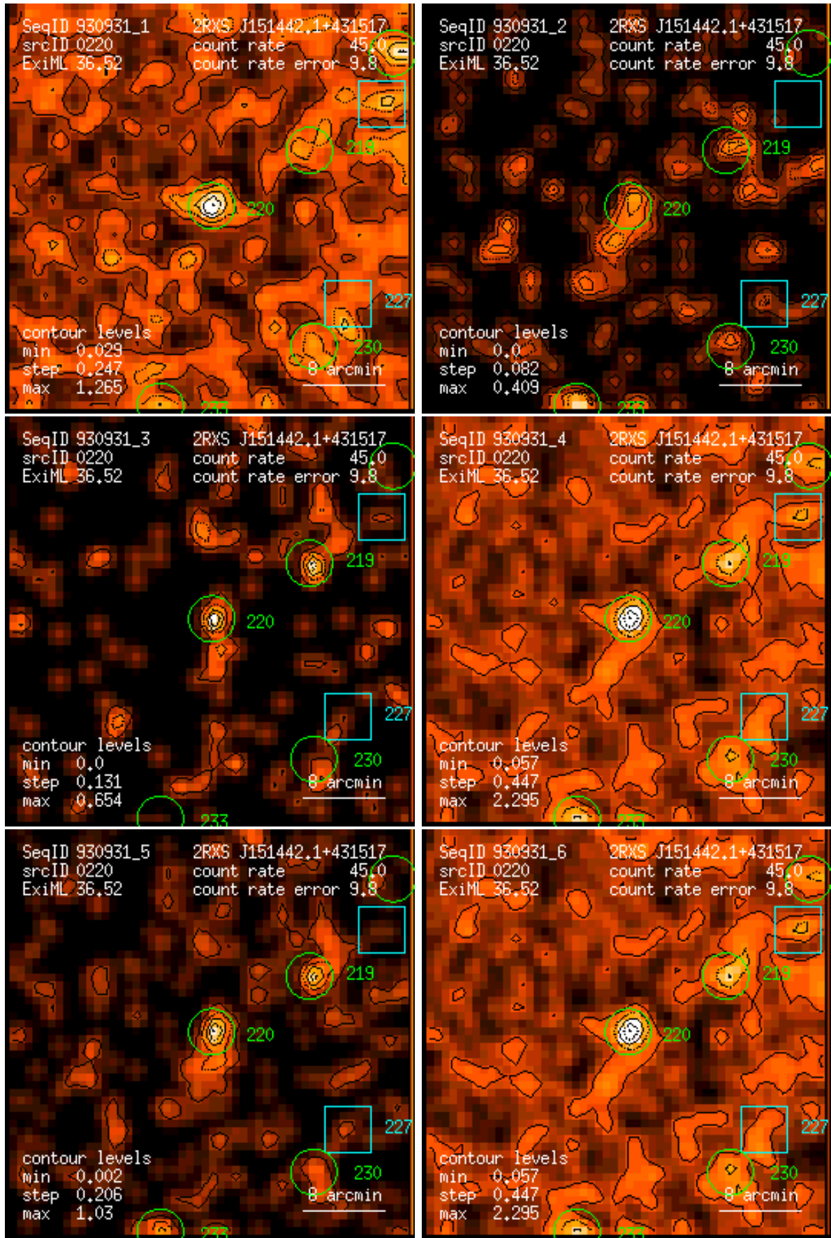
Figure 220: RASS 930931: detection 0220: band rate images, Gaussian filter: (1) PSPC channels 11 – 41, (2) 52 – 90, (3) 91 – 201, (4) 11 – 235, (5) 52 – 201, (6) 11 – 201. Broad band rates in counts/ks. Band rate contour levels in counts/ks/arcmin 2 .
