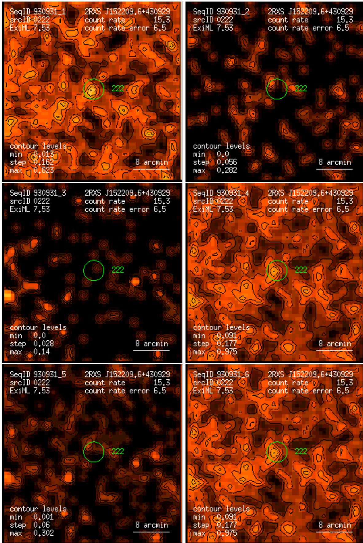
Figure 222: RASS 930931: detection 0222: band rate images, Gaussian filter: (1) PSPC channels 11 – 41, (2) 52 – 90, (3) 91 – 201, (4) 11 – 235, (5) 52 – 201, (6) 11 – 201. Broad band rates in counts/ks. Band rate contour levels in counts/ks/arcmin 2 .
