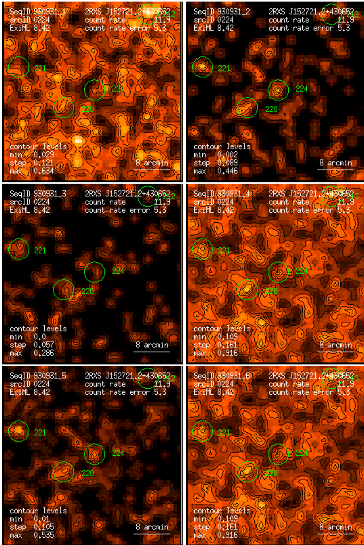
Figure 224: RASS 930931: detection 0224: band rate images, Gaussian filter: (1) PSPC channels 11 – 41, (2) 52 – 90, (3) 91 – 201, (4) 11 – 235, (5) 52 – 201, (6) 11 – 201. Broad band rates in counts/ks. Band rate contour levels in counts/ks/arcmin 2 .
