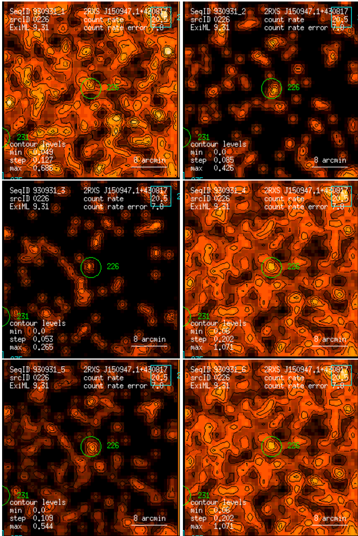
Figure 226: RASS 930931: detection 0226: band rate images, Gaussian filter: (1) PSPC channels 11 – 41, (2) 52 – 90, (3) 91 – 201, (4) 11 – 235, (5) 52 – 201, (6) 11 – 201. Broad band rates in counts/ks. Band rate contour levels in counts/ks/arcmin 2 .
