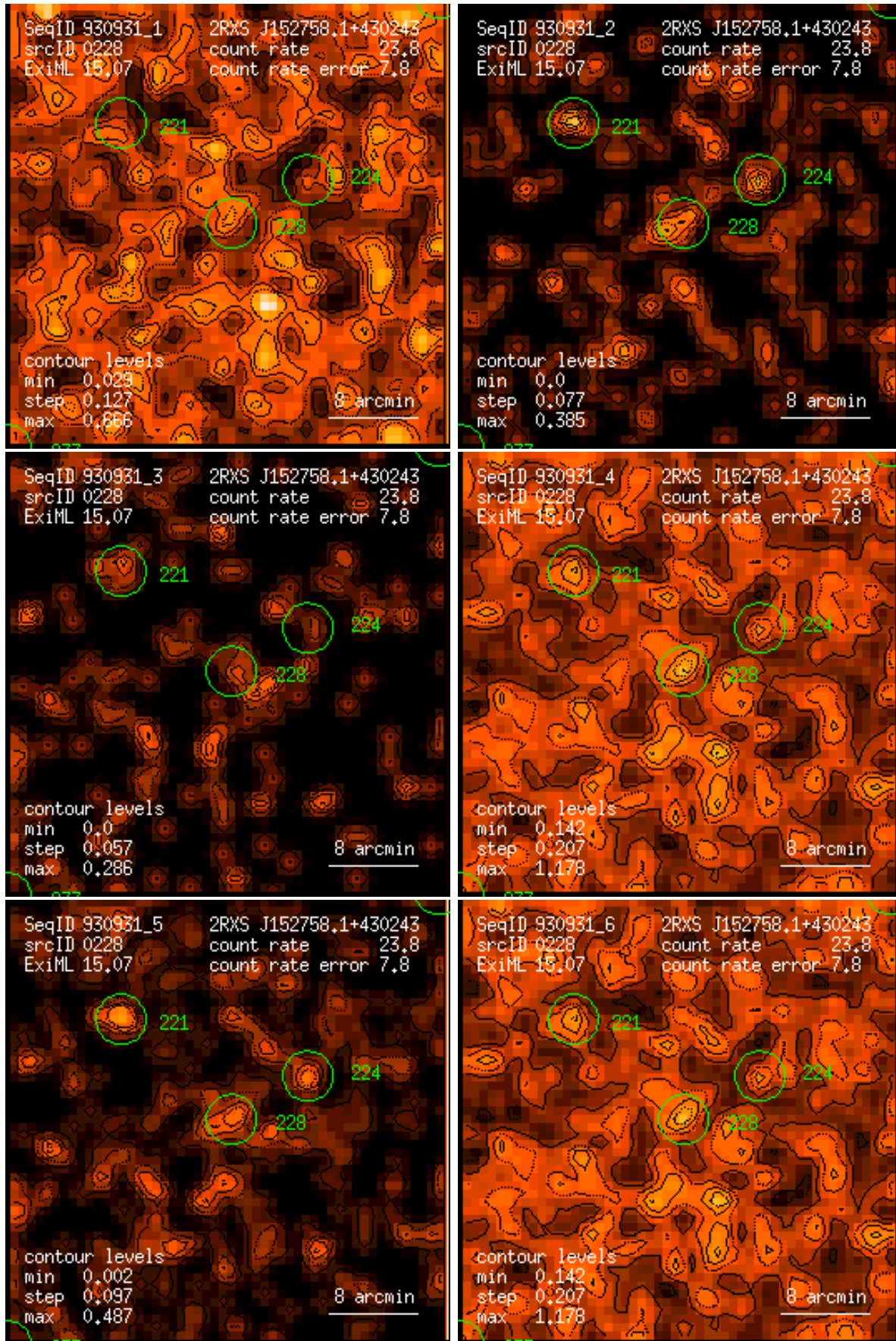
Figure 228: RASS 930931: detection 0228: band rate images, Gaussian filter: (1) PSPC channels 11 – 41, (2) 52 – 90, (3) 91 – 201, (4) 11 – 235, (5) 52 – 201, (6) 11 – 201. Broad band rates in counts/ks. Band rate contour levels in counts/ks/arcmin 2 .
