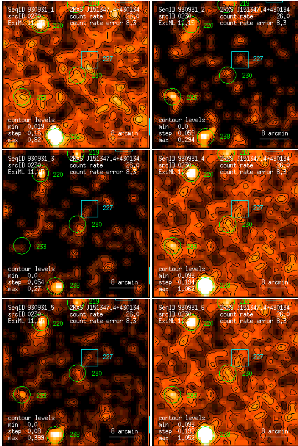
Figure 230: RASS 930931: detection 0230: band rate images, Gaussian filter: (1) PSPC channels 11 – 41, (2) 52 – 90, (3) 91 – 201, (4) 11 – 235, (5) 52 – 201, (6) 11 – 201. Broad band rates in counts/ks. Band rate contour levels in counts/ks/arcmin 2 .
