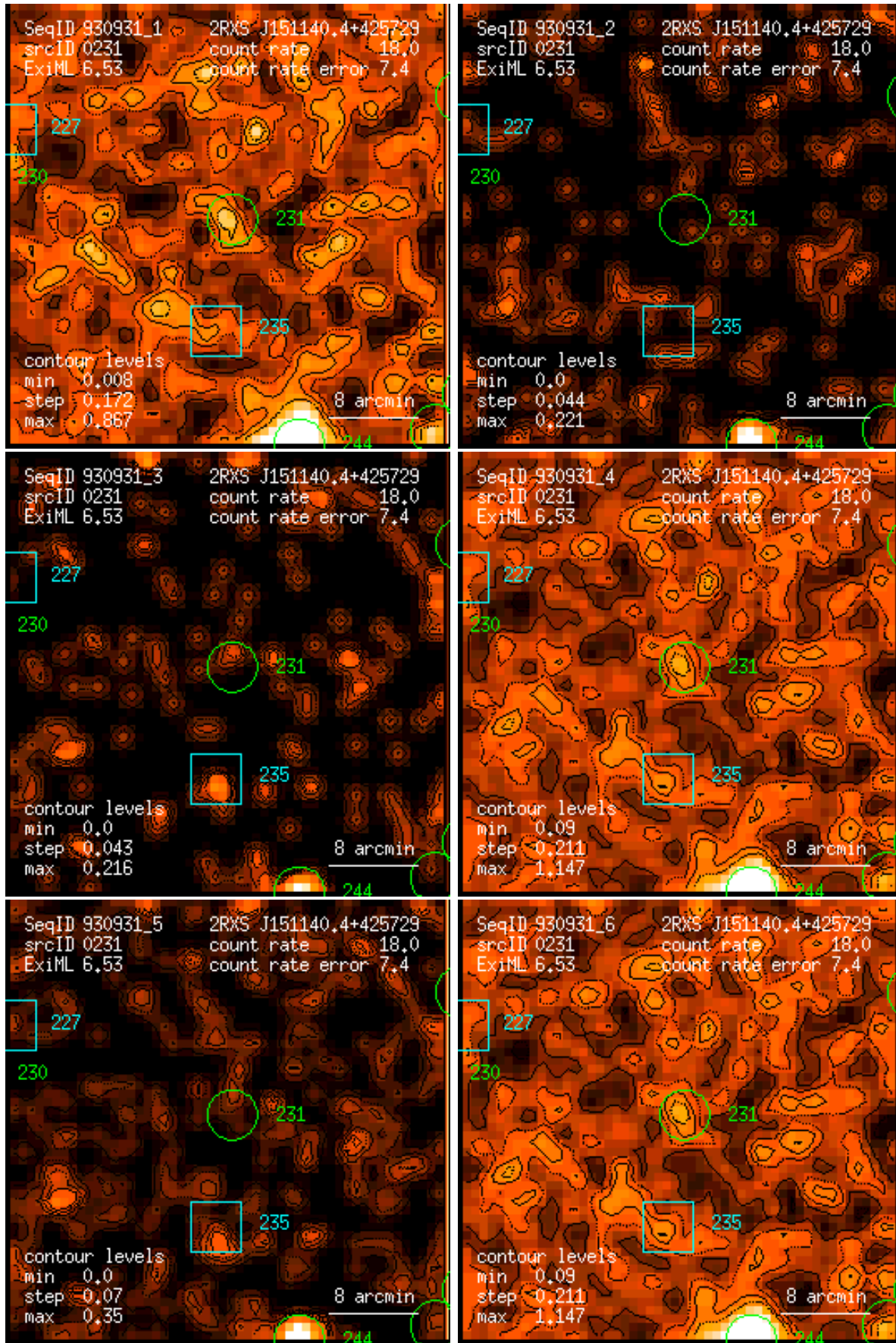
Figure 231: RASS 930931: detection 0231: band rate images, Gaussian filter: (1) PSPC channels 11 – 41, (2) 52 – 90, (3) 91 – 201, (4) 11 – 235, (5) 52 – 201, (6) 11 – 201. Broad band rates in counts/ks. Band rate contour levels in counts/ks/arcmin 2 .
