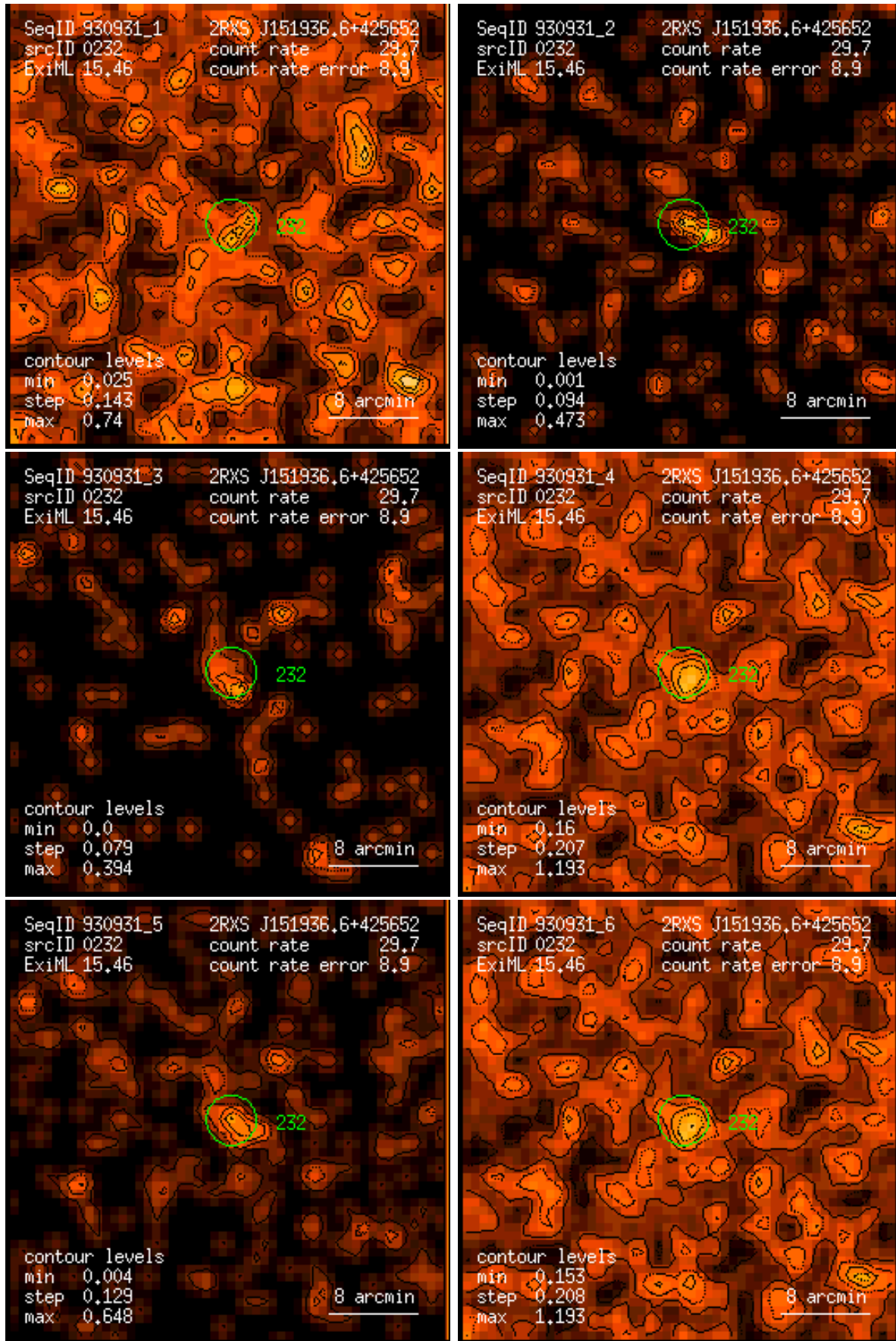
Figure 232: RASS 930931: detection 0232: band rate images, Gaussian filter: (1) PSPC channels 11 – 41, (2) 52 – 90, (3) 91 – 201, (4) 11 – 235, (5) 52 – 201, (6) 11 – 201. Broad band rates in counts/ks. Band rate contour levels in counts/ks/arcmin 2 .
