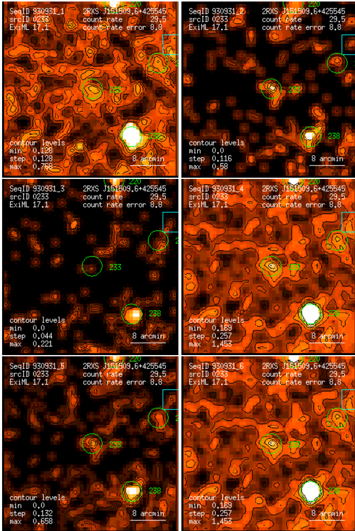
Figure 233: RASS 930931: detection 0233: band rate images, Gaussian filter: (1) PSPC channels 11 – 41, (2) 52 – 90, (3) 91 – 201, (4) 11 – 235, (5) 52 – 201, (6) 11 – 201. Broad band rates in counts/ks. Band rate contour levels in counts/ks/arcmin 2 .
