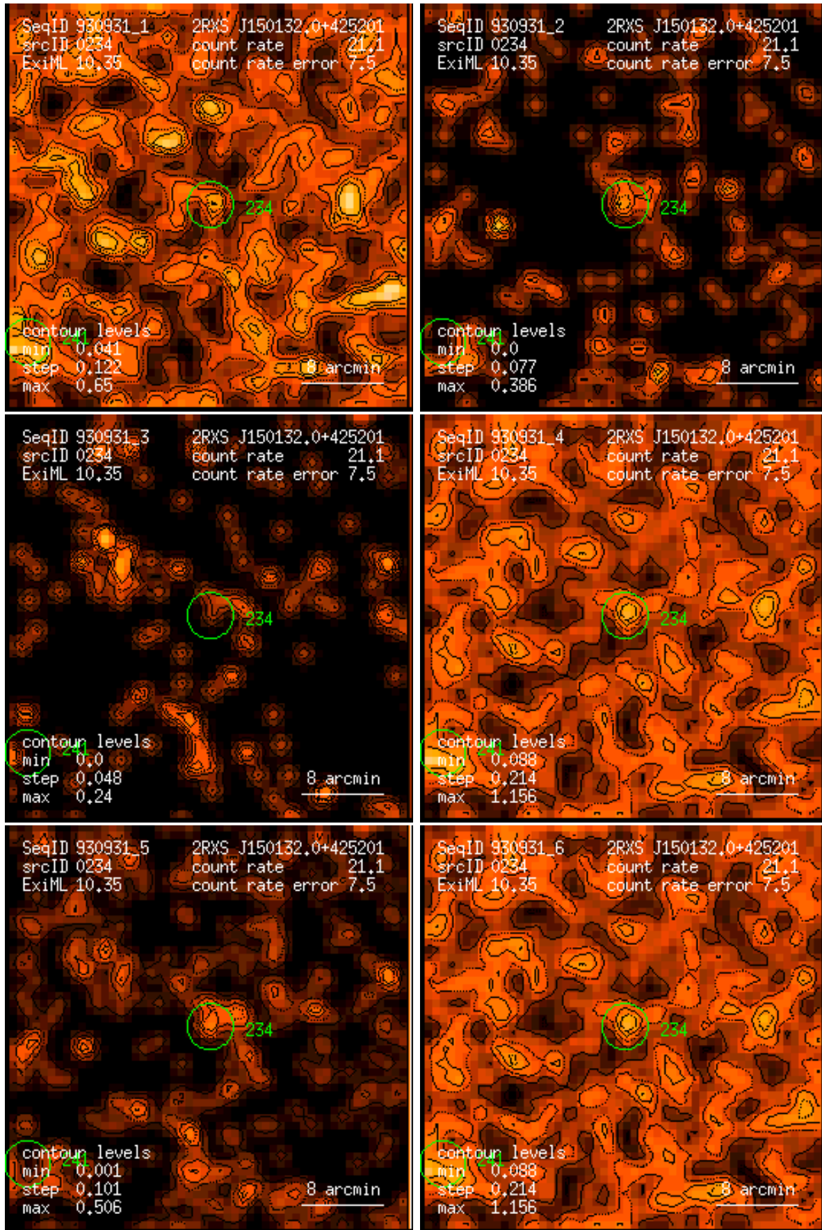
Figure 234: RASS 930931: detection 0234: band rate images, Gaussian filter: (1) PSPC channels 11 – 41, (2) 52 – 90, (3) 91 – 201, (4) 11 – 235, (5) 52 – 201, (6) 11 – 201. Broad band rates in counts/ks. Band rate contour levels in counts/ks/arcmin 2 .
