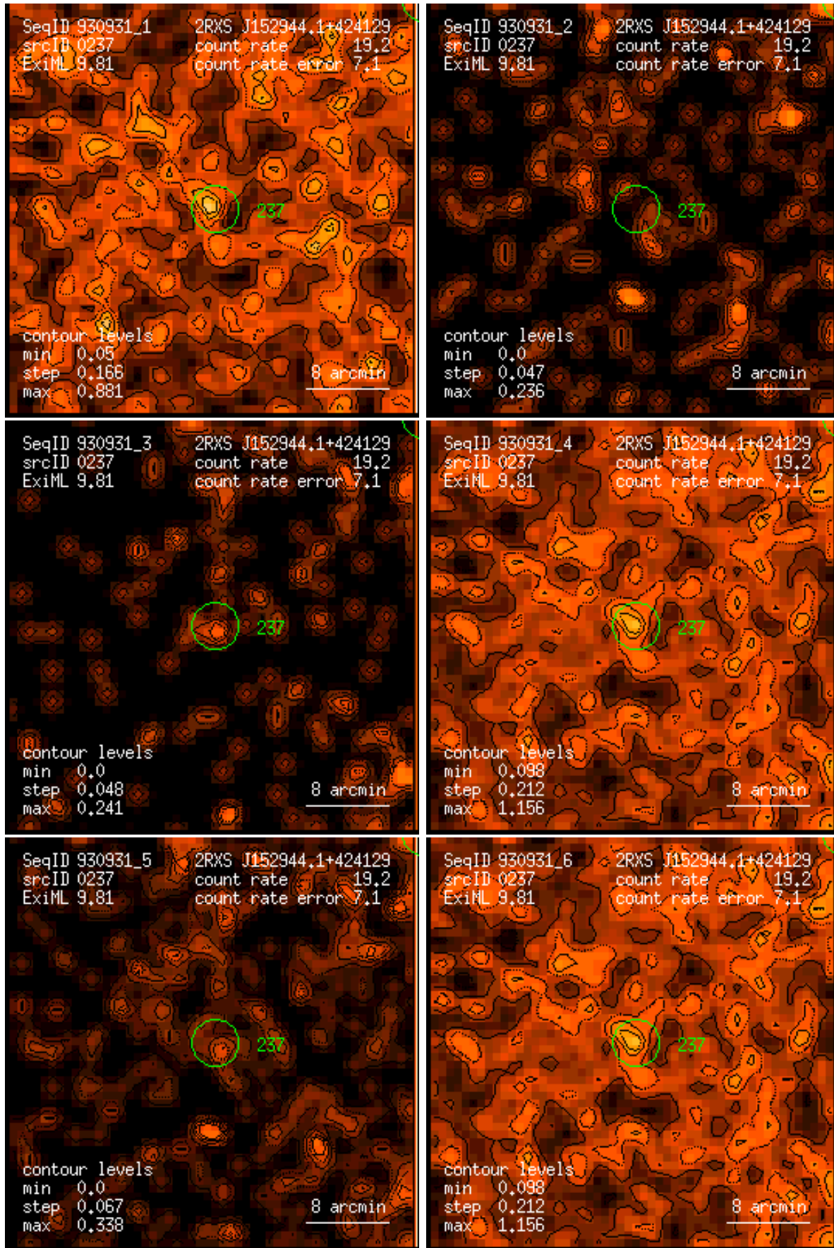
Figure 237: RASS 930931: detection 0237: band rate images, Gaussian filter: (1) PSPC channels 11 – 41, (2) 52 – 90, (3) 91 – 201, (4) 11 – 235, (5) 52 – 201, (6) 11 – 201. Broad band rates in counts/ks. Band rate contour levels in counts/ks/arcmin 2 .
