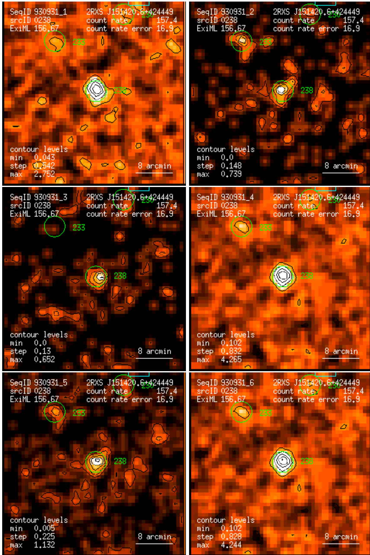
Figure 238: RASS 930931: detection 0238: band rate images, Gaussian filter: (1) PSPC channels 11 – 41, (2) 52 – 90, (3) 91 – 201, (4) 11 – 235, (5) 52 – 201, (6) 11 – 201. Broad band rates in counts/ks. Band rate contour levels in counts/ks/arcmin 2 .
