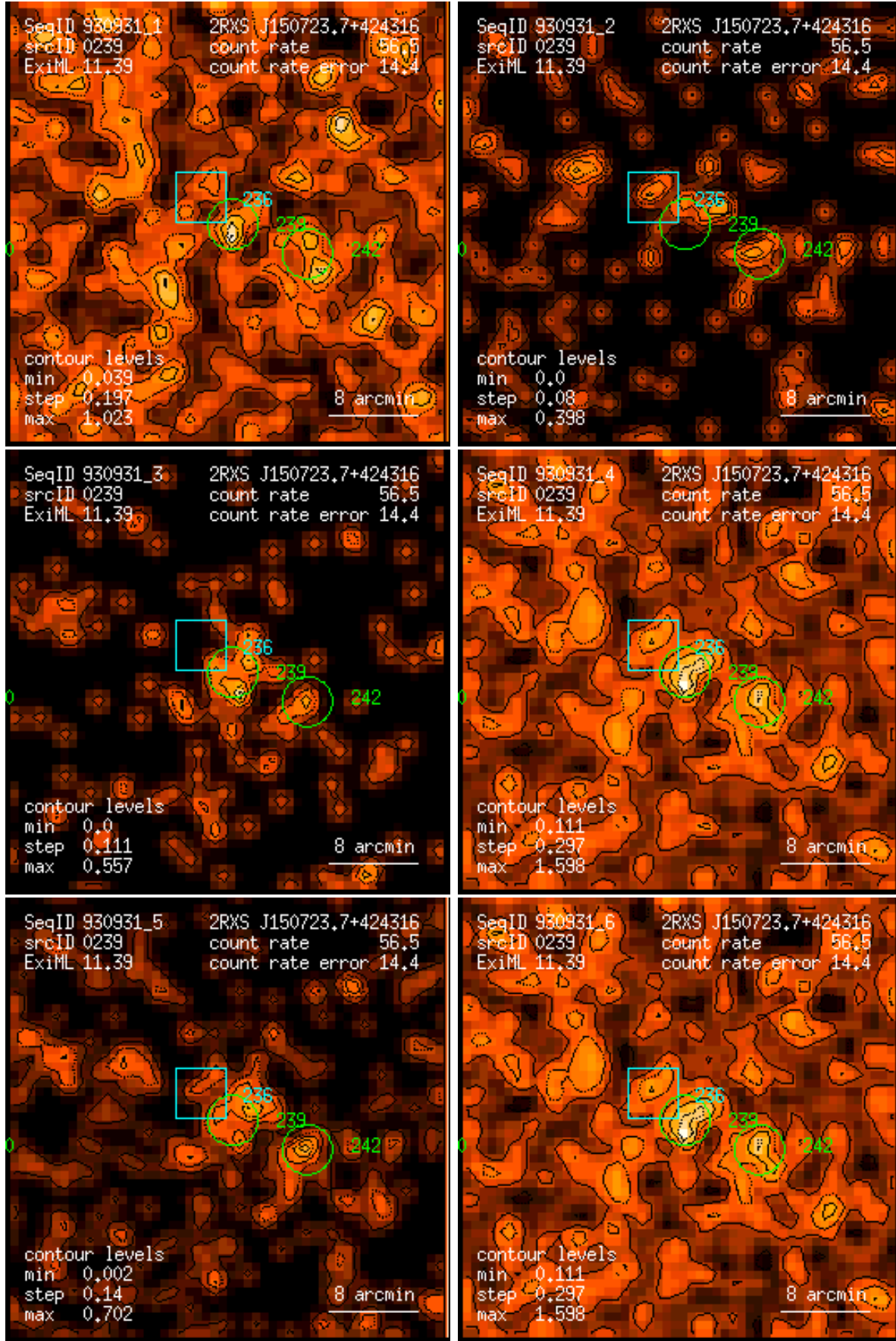
Figure 239: RASS 930931: detection 0239: band rate images, Gaussian filter: (1) PSPC channels 11 – 41, (2) 52 – 90, (3) 91 – 201, (4) 11 – 235, (5) 52 – 201, (6) 11 – 201. Broad band rates in counts/ks. Band rate contour levels in counts/ks/arcmin 2 .
