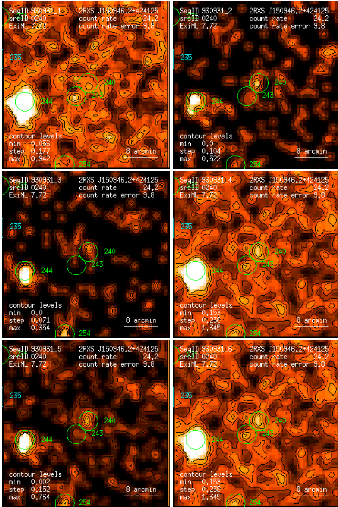
Figure 240: RASS 930931: detection 0240: band rate images, Gaussian filter: (1) PSPC channels 11 – 41, (2) 52 – 90, (3) 91 – 201, (4) 11 – 235, (5) 52 – 201, (6) 11 – 201. Broad band rates in counts/ks. Band rate contour levels in counts/ks/arcmin 2 .
