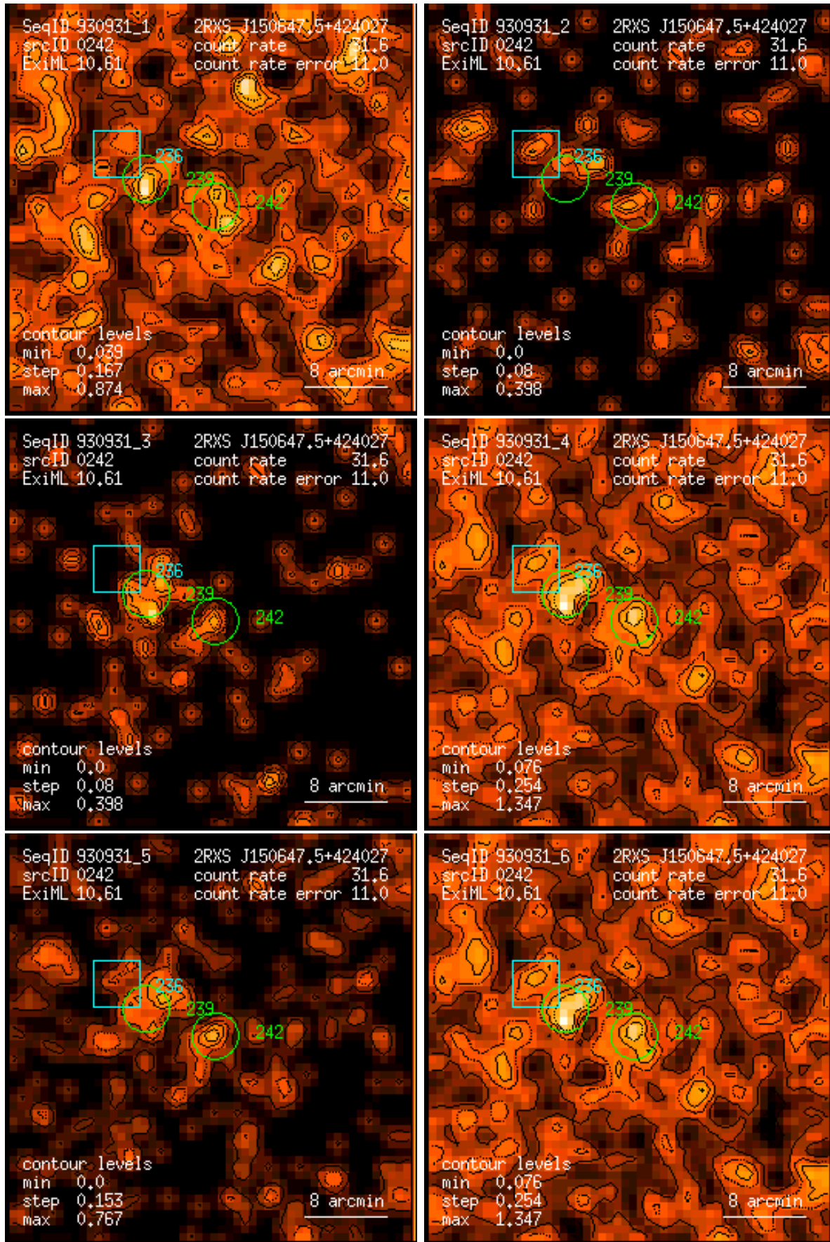
Figure 242: RASS 930931: detection 0242: band rate images, Gaussian filter: (1) PSPC channels 11 – 41, (2) 52 – 90, (3) 91 – 201, (4) 11 – 235, (5) 52 – 201, (6) 11 – 201. Broad band rates in counts/ks. Band rate contour levels in counts/ks/arcmin 2 .
