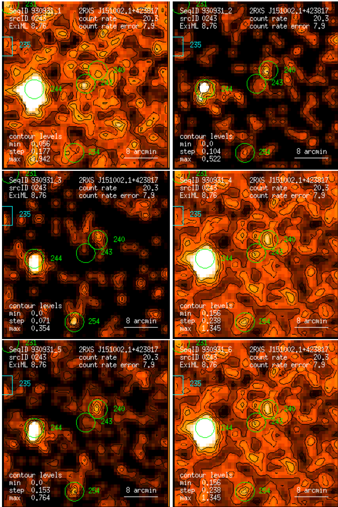
Figure 243: RASS 930931: detection 0243: band rate images, Gaussian filter: (1) PSPC channels 11 – 41, (2) 52 – 90, (3) 91 – 201, (4) 11 – 235, (5) 52 – 201, (6) 11 – 201. Broad band rates in counts/ks. Band rate contour levels in counts/ks/arcmin 2 .
