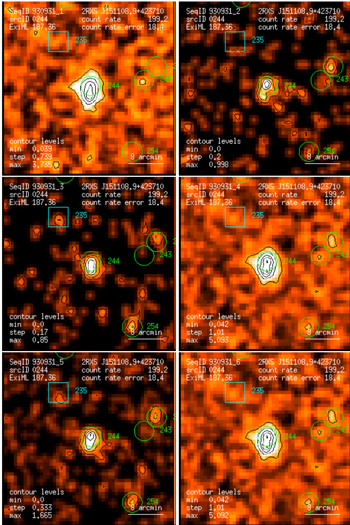
Figure 244: RASS 930931: detection 0244: band rate images, Gaussian filter: (1) PSPC channels 11 – 41, (2) 52 – 90, (3) 91 – 201, (4) 11 – 235, (5) 52 – 201, (6) 11 – 201. Broad band rates in counts/ks. Band rate contour levels in counts/ks/arcmin 2 .
