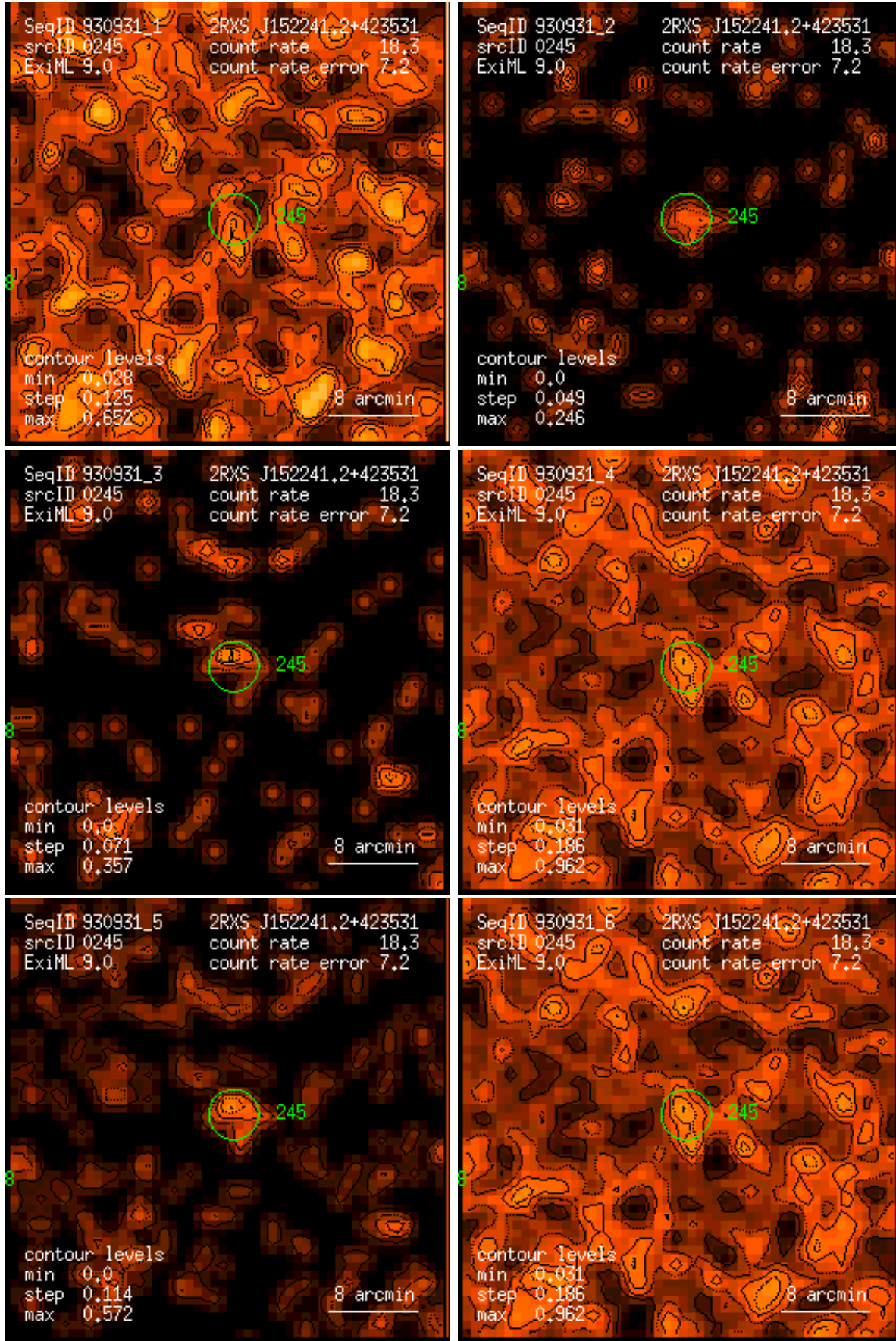
Figure 245: RASS 930931: detection 0245: band rate images, Gaussian filter: (1) PSPC channels 11 – 41, (2) 52 – 90, (3) 91 – 201, (4) 11 – 235, (5) 52 – 201, (6) 11 – 201. Broad band rates in counts/ks. Band rate contour levels in counts/ks/arcmin 2 .
