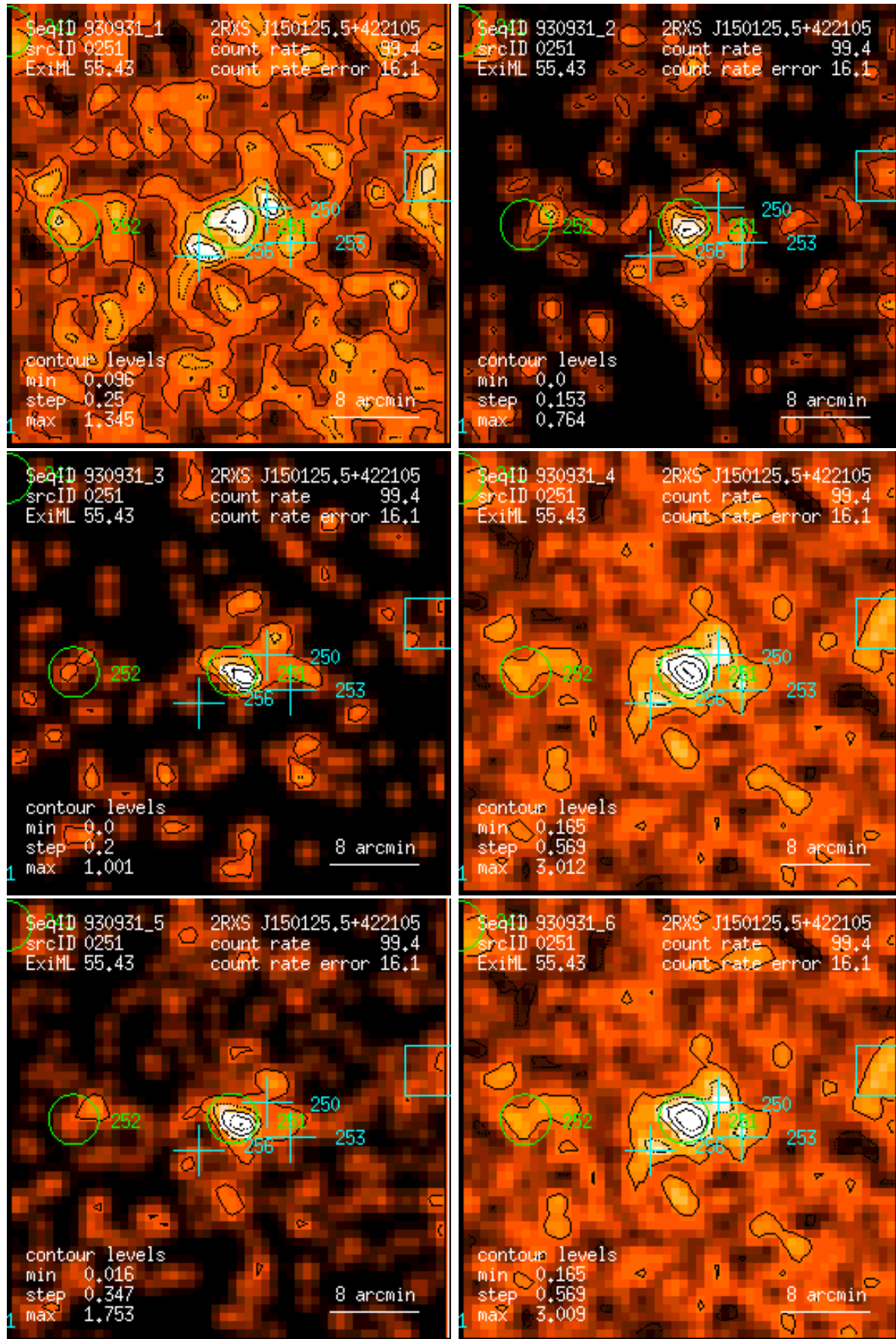
Figure 251: RASS 930931: detection 0251: band rate images, Gaussian filter: (1) PSPC channels 11 – 41, (2) 52 – 90, (3) 91 – 201, (4) 11 – 235, (5) 52 – 201, (6) 11 – 201. Broad band rates in counts/ks. Band rate contour levels in counts/ks/arcmin 2 .
