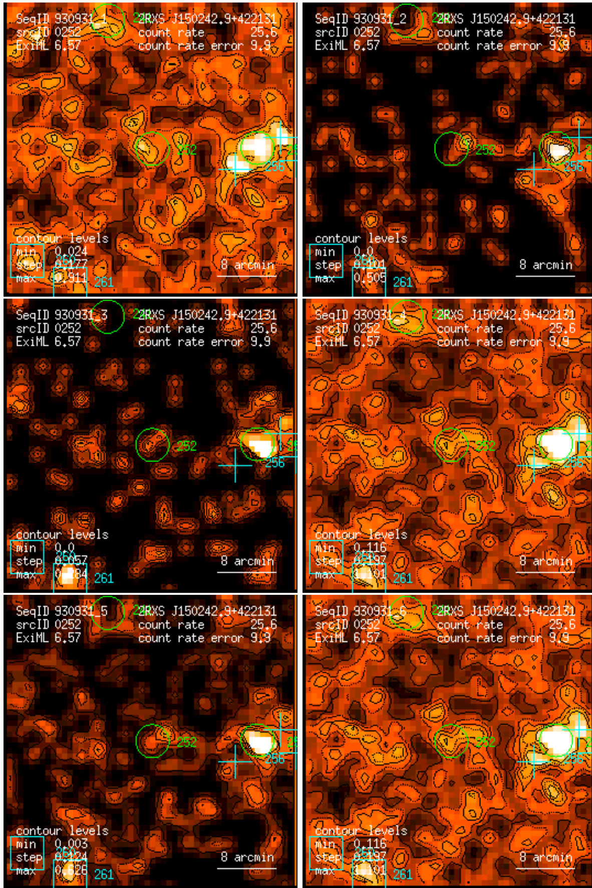
Figure 252: RASS 930931: detection 0252: band rate images, Gaussian filter: (1) PSPC channels 11 – 41, (2) 52 – 90, (3) 91 – 201, (4) 11 – 235, (5) 52 – 201, (6) 11 – 201. Broad band rates in counts/ks. Band rate contour levels in counts/ks/arcmin 2 .
