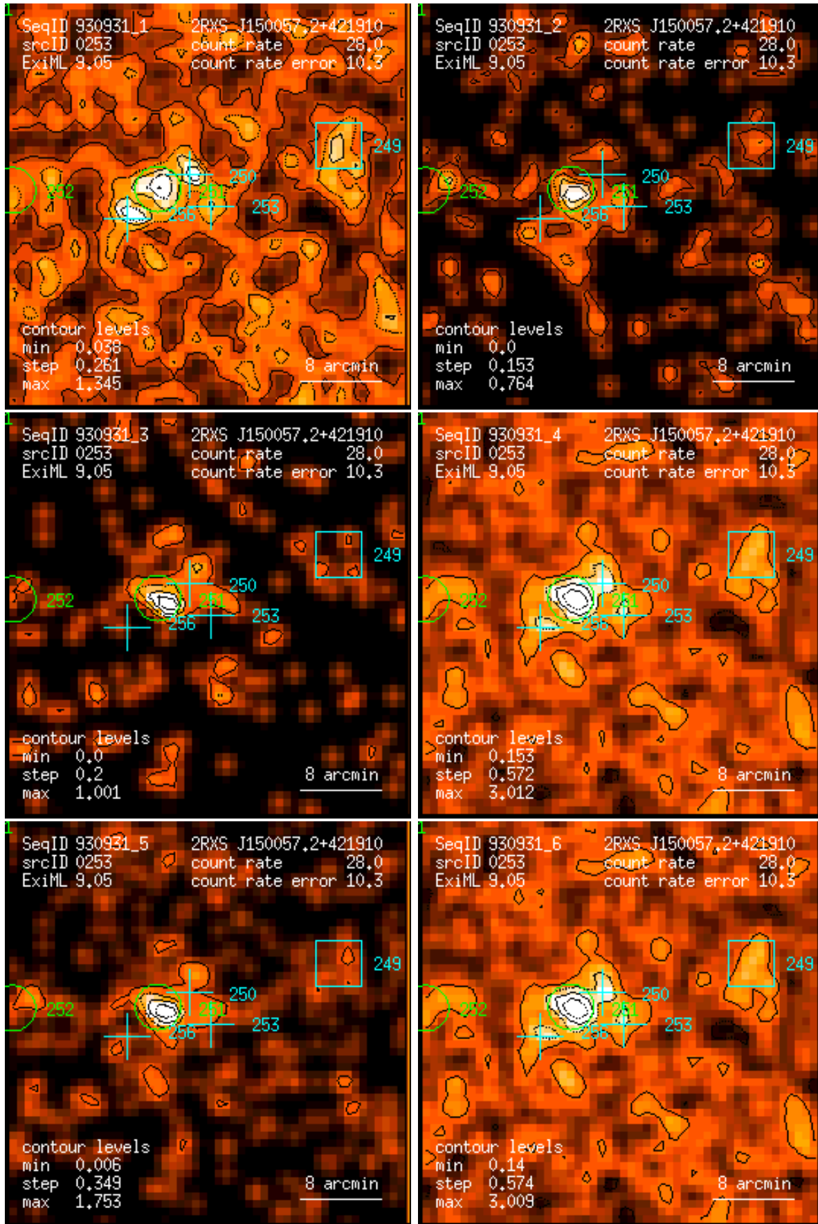
Figure 253: RASS 930931: detection 0253: band rate images, Gaussian filter: (1) PSPC channels 11 – 41, (2) 52 – 90, (3) 91 – 201, (4) 11 – 235, (5) 52 – 201, (6) 11 – 201. Broad band rates in counts/ks. Band rate contour levels in counts/ks/arcmin 2 .
