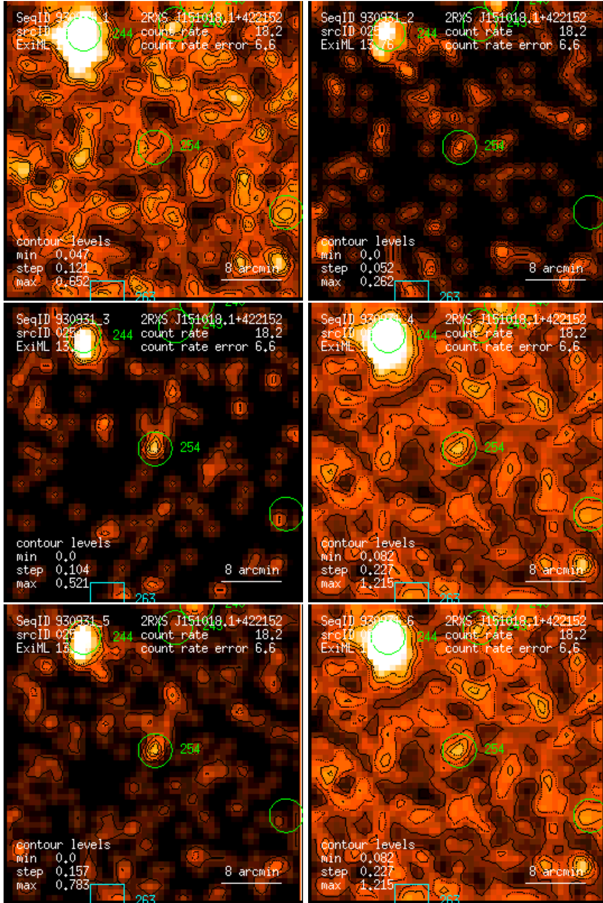
Figure 254: RASS 930931: detection 0254: band rate images, Gaussian filter: (1) PSPC channels 11 – 41, (2) 52 – 90, (3) 91 – 201, (4) 11 – 235, (5) 52 – 201, (6) 11 – 201. Broad band rates in counts/ks. Band rate contour levels in counts/ks/arcmin 2 .
