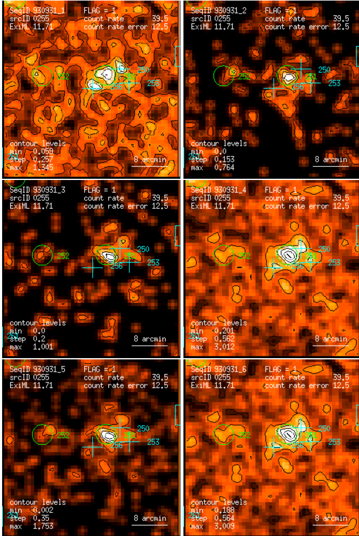
Figure 255: RASS 930931: detection 0255: band rate images, Gaussian filter: (1) PSPC channels 11 – 41, (2) 52 – 90, (3) 91 – 201, (4) 11 – 235, (5) 52 – 201, (6) 11 – 201. Broad band rates in counts/ks. Band rate contour levels in counts/ks/arcmin 2 .
