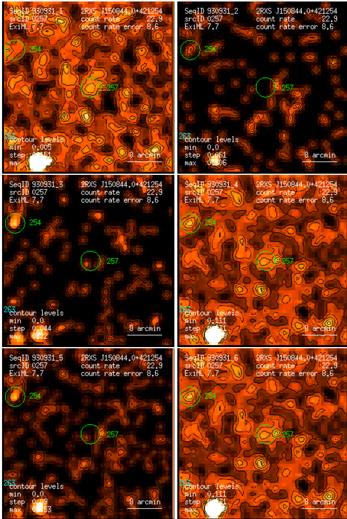
Figure 257: RASS 930931: detection 0257: band rate images, Gaussian filter: (1) PSPC channels 11 – 41, (2) 52 – 90, (3) 91 – 201, (4) 11 – 235, (5) 52 – 201, (6) 11 – 201. Broad band rates in counts/ks. Band rate contour levels in counts/ks/arcmin 2 .
