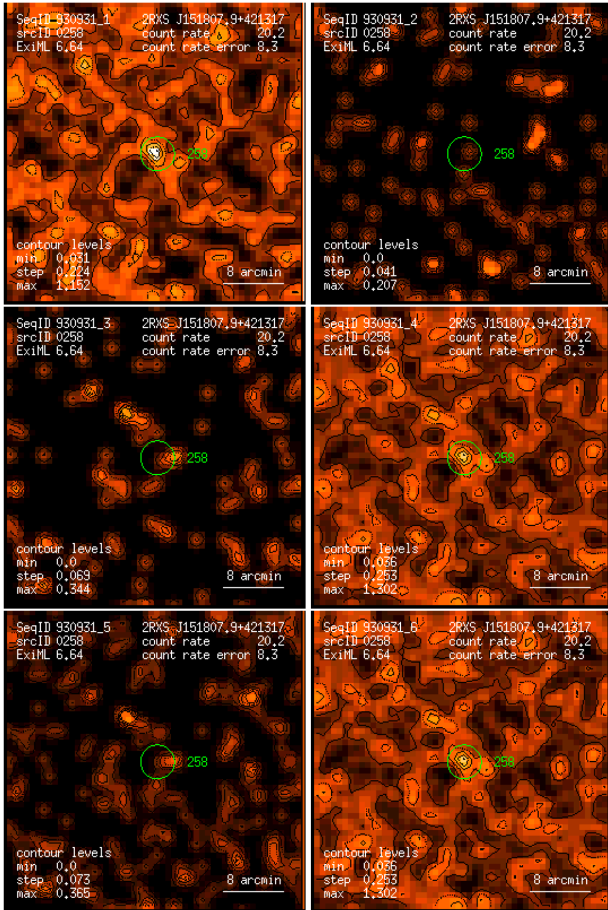
Figure 258: RASS 930931: detection 0258: band rate images, Gaussian filter: (1) PSPC channels 11 – 41, (2) 52 – 90, (3) 91 – 201, (4) 11 – 235, (5) 52 – 201, (6) 11 – 201. Broad band rates in counts/ks. Band rate contour levels in counts/ks/arcmin 2 .
