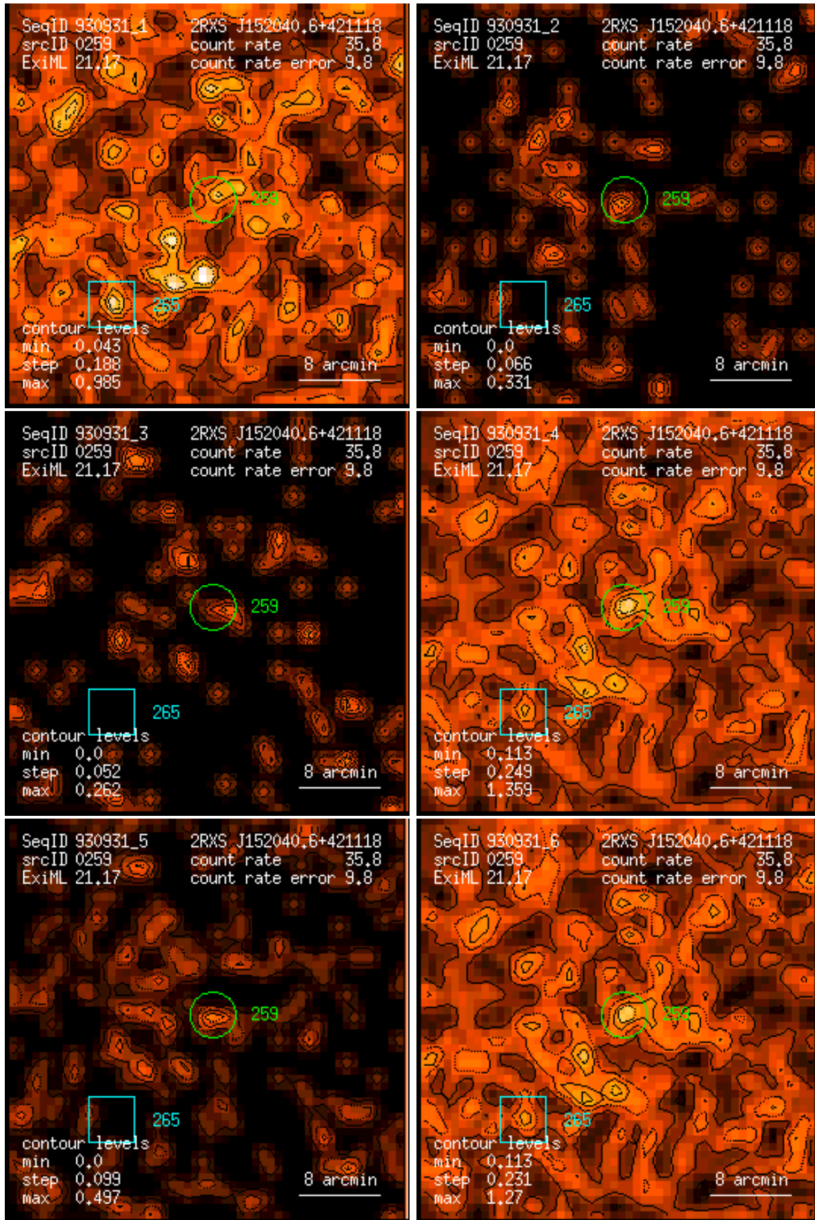
Figure 259: RASS 930931: detection 0259: band rate images, Gaussian filter: (1) PSPC channels 11 – 41, (2) 52 – 90, (3) 91 – 201, (4) 11 – 235, (5) 52 – 201, (6) 11 – 201. Broad band rates in counts/ks. Band rate contour levels in counts/ks/arcmin 2 .
