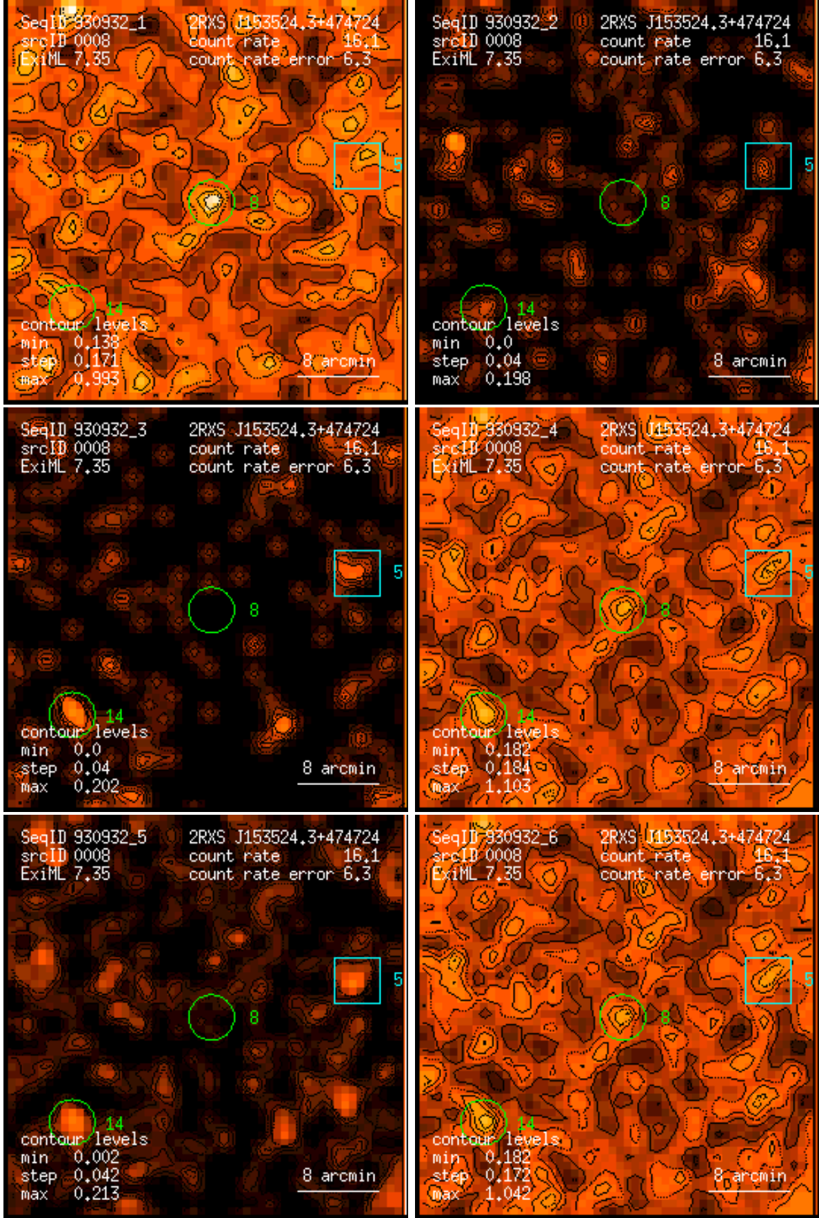
Figure 8: RASS 930932: detection 0008: band rate images, Gaussian filter: (1) PSPC channels 11 – 41, (2) 52 – 90, (3) 91 – 201, (4) 11 – 235, (5) 52 – 201, (6) 11 – 201. Broad band rates in counts/ks. Band rate contour levels in counts/ks/arcmin 2 .
