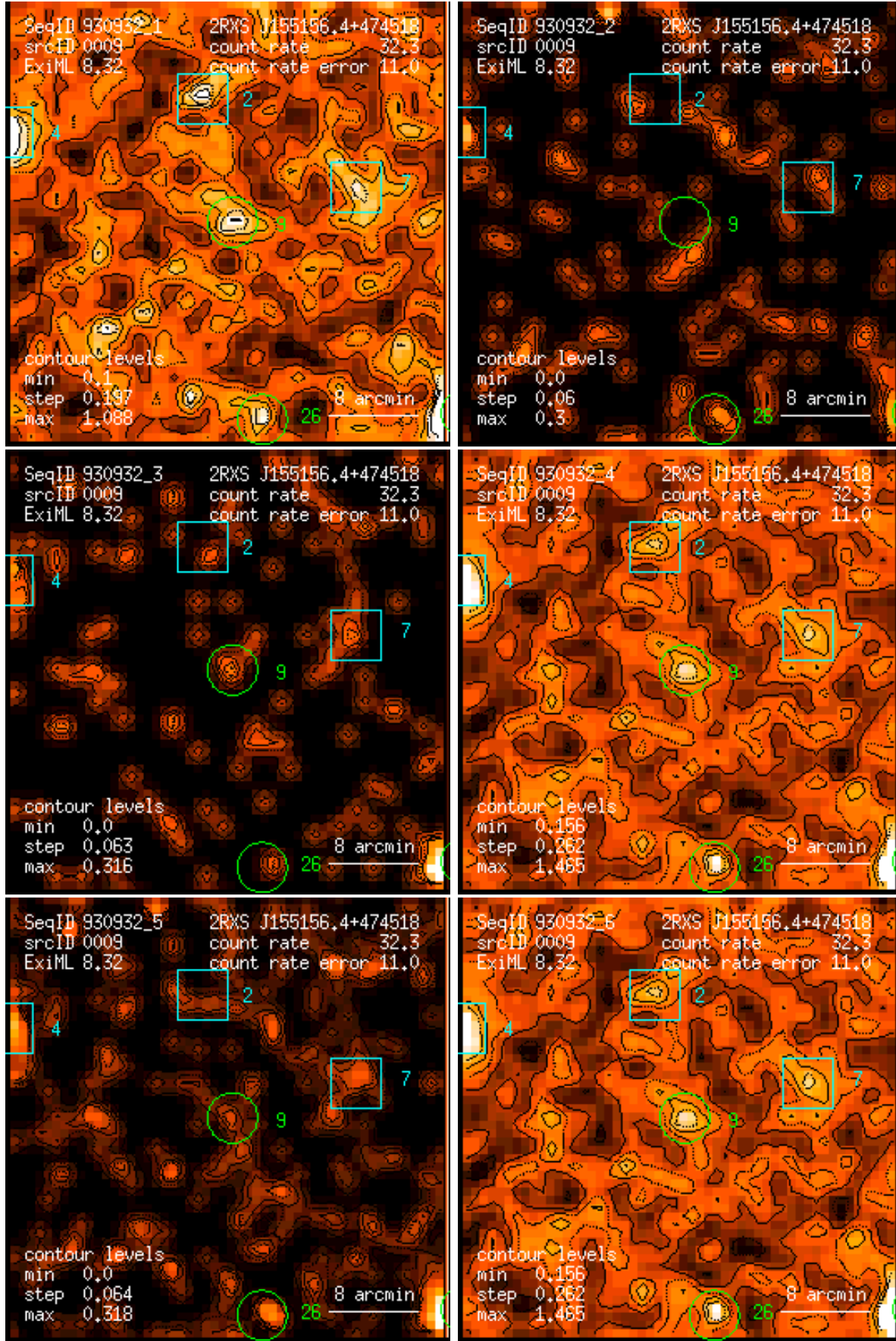
Figure 9: RASS 930932: detection 0009: band rate images, Gaussian filter: (1) PSPC channels 11 – 41, (2) 52 – 90, (3) 91 – 201, (4) 11 – 235, (5) 52 – 201, (6) 11 – 201. Broad band rates in counts/ks. Band rate contour levels in counts/ks/arcmin 2 .
