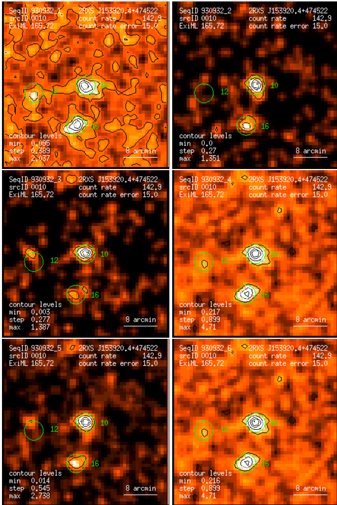
Figure 10: RASS 930932: detection 0010: band rate images, Gaussian filter: (1) PSPC channels 11 – 41, (2) 52 – 90, (3) 91 – 201, (4) 11 – 235, (5) 52 – 201, (6) 11 – 201. Broad band rates in counts/ks. Band rate contour levels in counts/ks/arcmin 2 .
