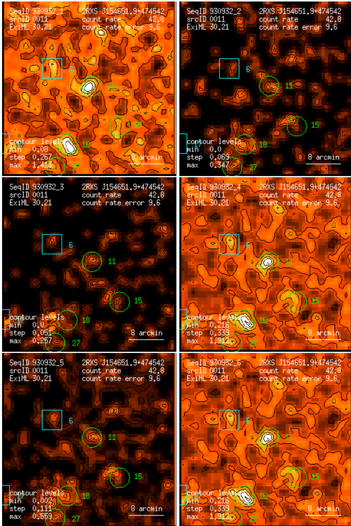
Figure 11: RASS 930932: detection 0011: band rate images, Gaussian filter: (1) PSPC channels 11 – 41, (2) 52 – 90, (3) 91 – 201, (4) 11 – 235, (5) 52 – 201, (6) 11 – 201. Broad band rates in counts/ks. Band rate contour levels in counts/ks/arcmin 2 .
