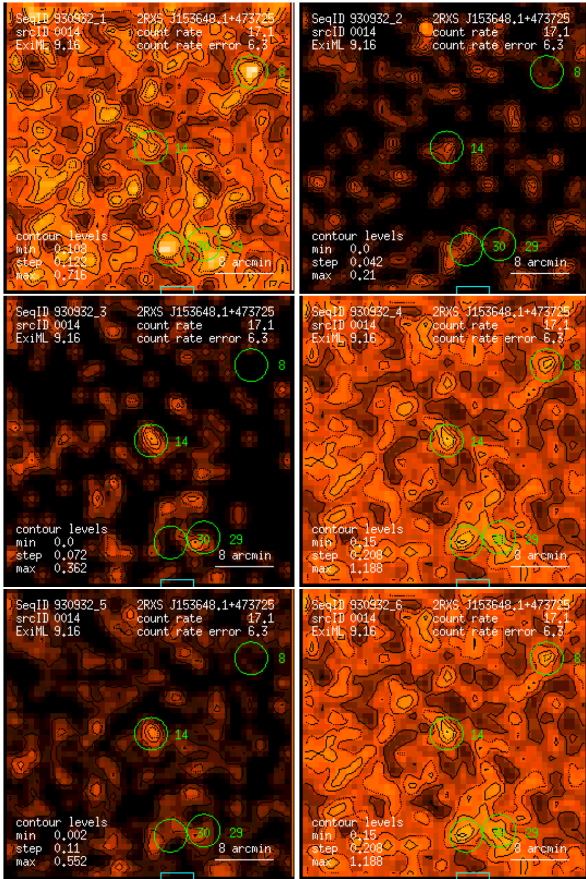
Figure 14: RASS 930932: detection 0014: band rate images, Gaussian filter: (1) PSPC channels 11 – 41, (2) 52 – 90, (3) 91 – 201, (4) 11 – 235, (5) 52 – 201, (6) 11 – 201. Broad band rates in counts/ks. Band rate contour levels in counts/ks/arcmin 2 .
