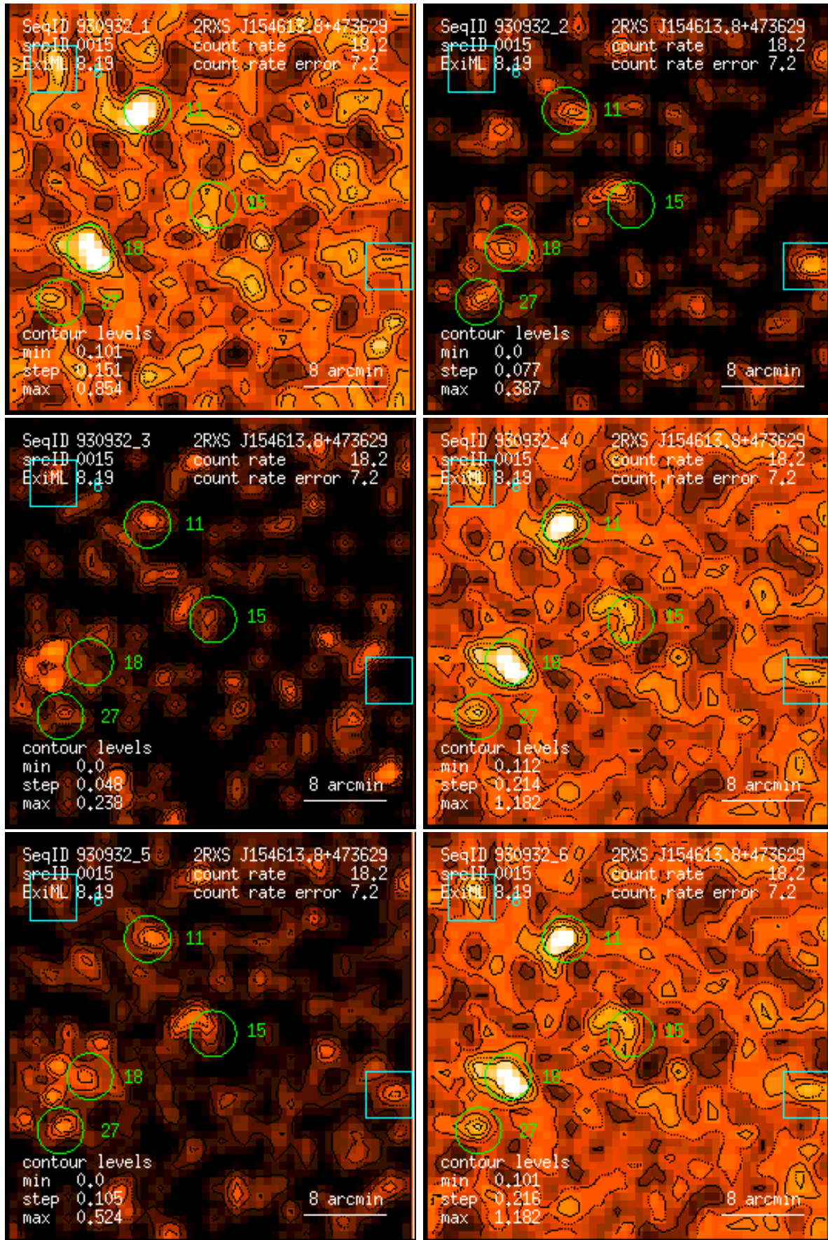
Figure 15: RASS 930932: detection 0015: band rate images, Gaussian filter: (1) PSPC channels 11 – 41, (2) 52 – 90, (3) 91 – 201, (4) 11 – 235, (5) 52 – 201, (6) 11 – 201. Broad band rates in counts/ks. Band rate contour levels in counts/ks/arcmin 2 .
